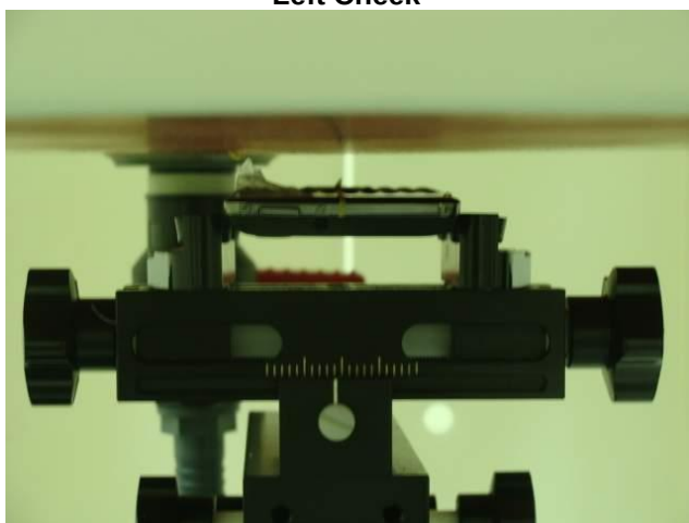
Front of the DUT with Phantom 1 cm Gap
