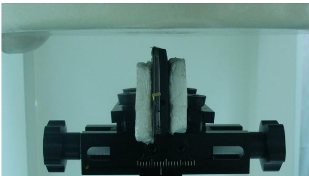
Left Side of the DUT with Phantom 1 cm Gap
