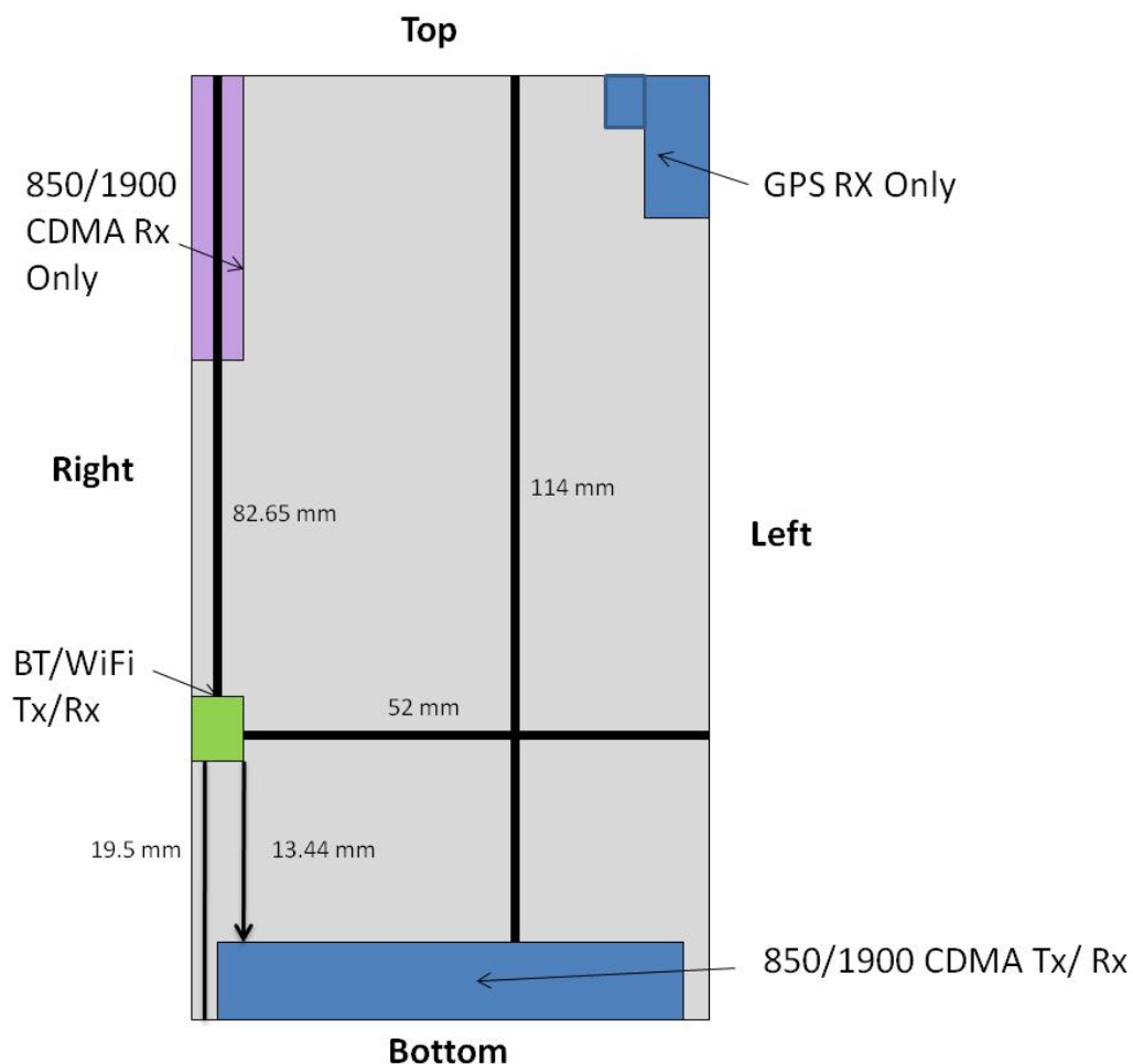
Figure 14-1 Identification of Sides for SAR Testing (Back View)
