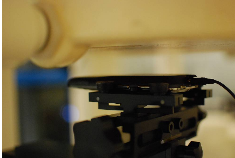
SAR Test Setup Photo 11 – Back at 2.5 cm
