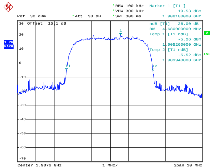
Higher Band Edge Plot on Channel 9538
