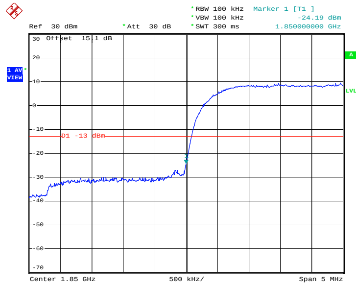
Lower Band Edge Plot on Channel 9262
