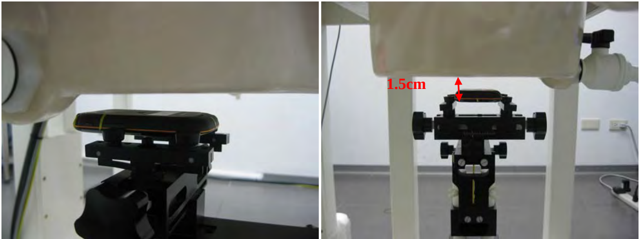
Fig.7 Body worn- EUT to flat phantom and distance between flat phantom and mobile phone is 1.5 cm.
