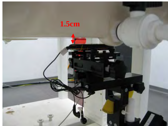
Fig.9 Body worn- EUT Back to flat phantom and distance between flat phantom and mobile phone is 1.5 cm. (with headset)
