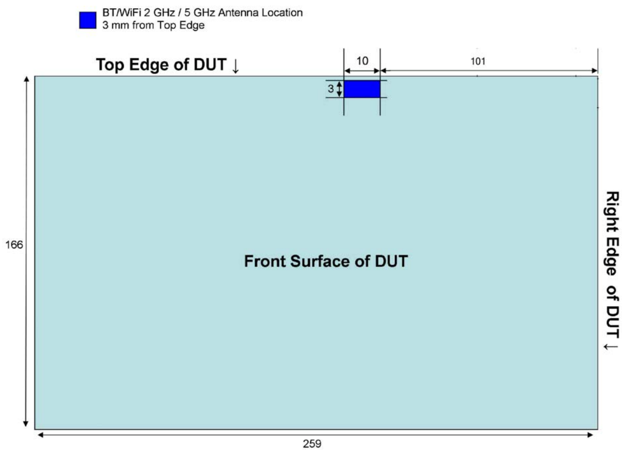
Figure 3: Device Dimensions and Antenna Separation Distances
