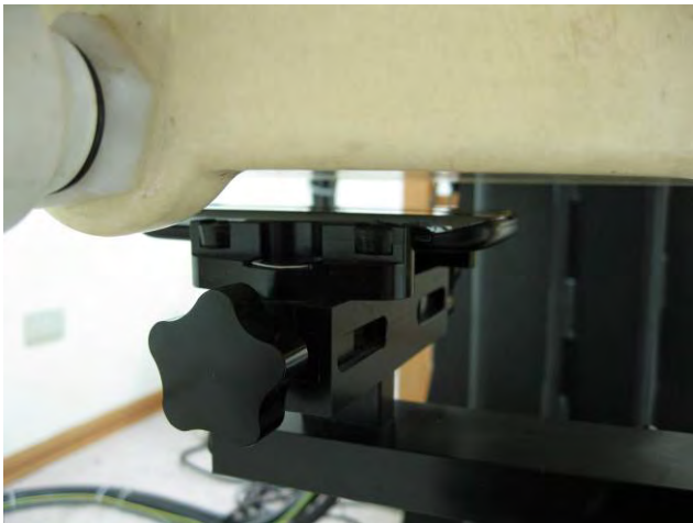
Fig.7 Hotsopt mode- EUT front to flat phantom and distance between flat phantom and mobile phone is 1 cm.
