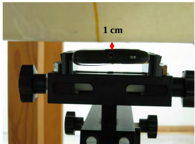
Fig.8 Hotsopt mode- EUT back to flat phantom and distance between flat phantom and mobile phone is 1 cm.
