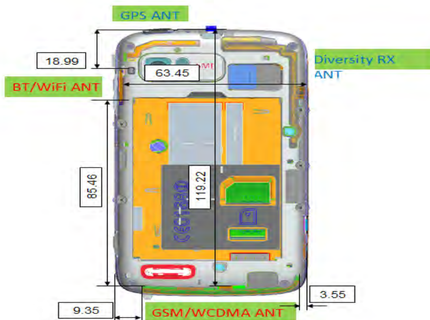
Fig.18 Antenna position of EUT
