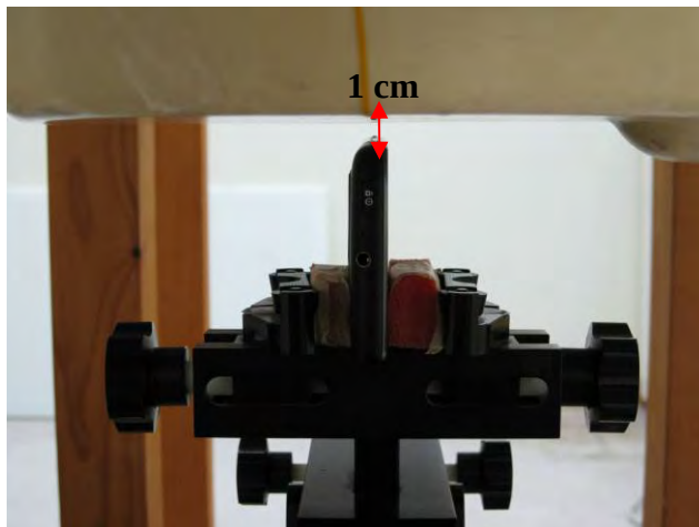
Fig.11 Hotsopt mode- EUT Right to flat phantom and distance between flat phantom and mobile phone is 1 cm.
