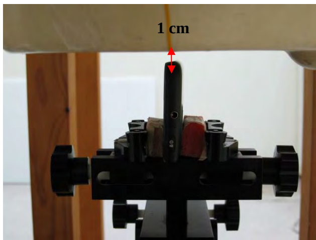
Fig.12 Hotsopt mode- EUT Left to flat phantom and distance between flat phantom and mobile phone is 1 cm.
