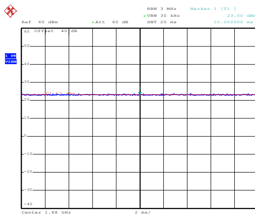
1880MHz - 80% AM
