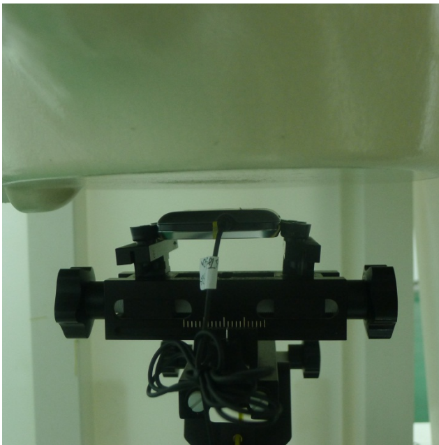
Back of the DUT with Phantom 1.5 cm Gap
