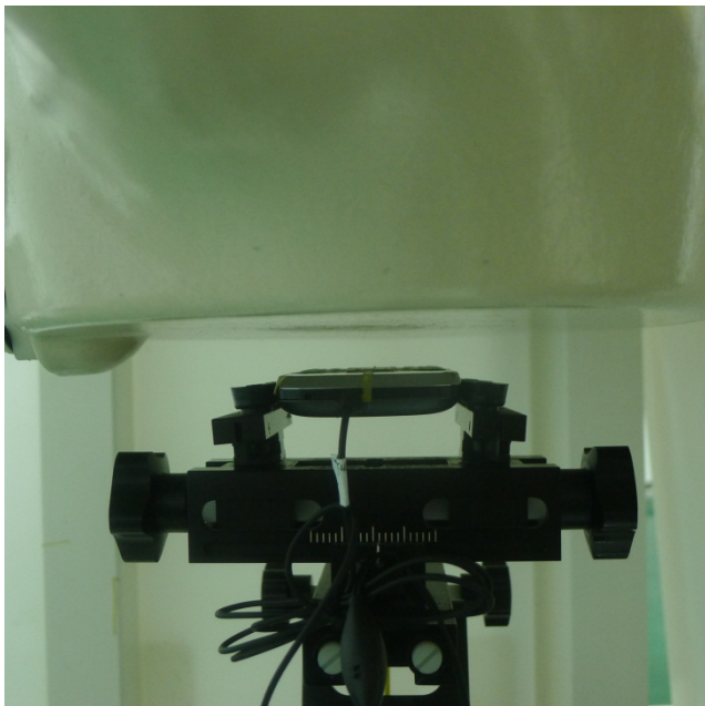
Front of the DUT with Phantom 1.5 cm Gap
