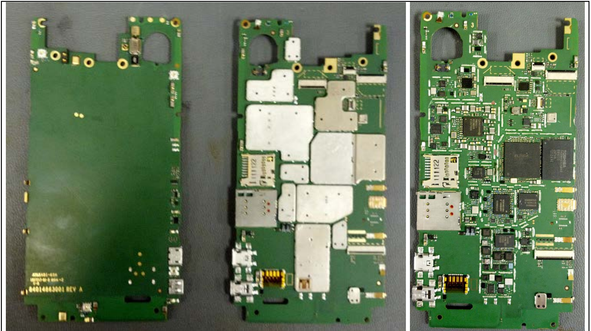
Photograph 9-2: Main PC Board, Shown with and without Shields in place (Component Side) and Non-Component Side.
