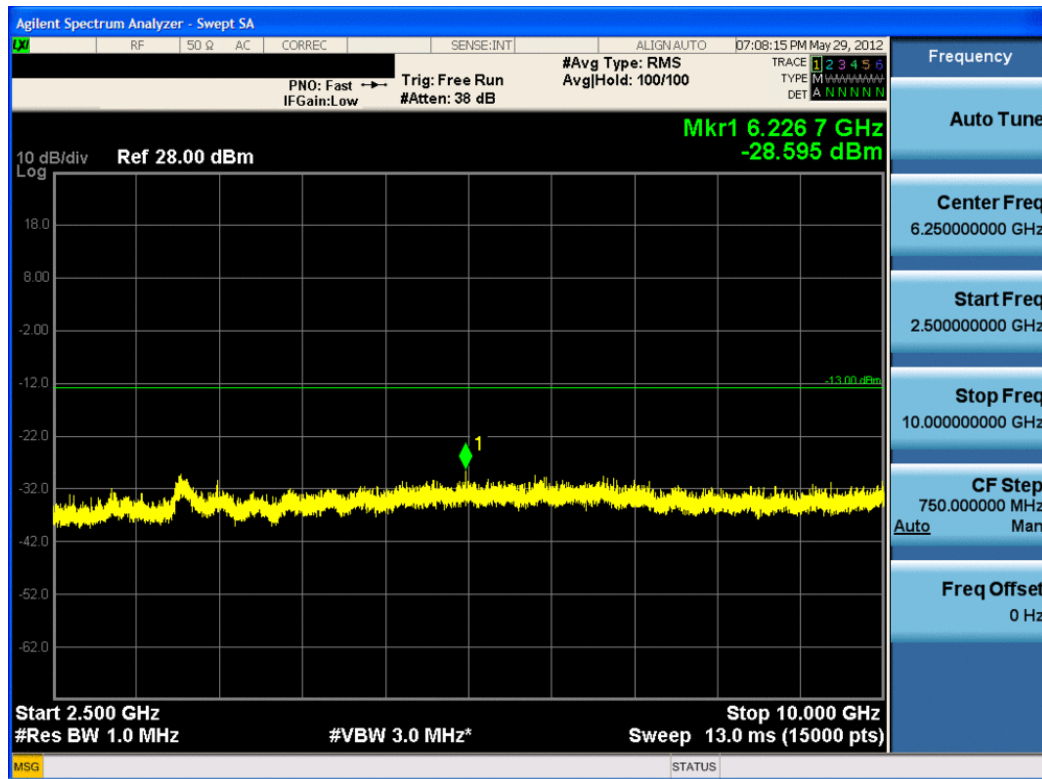
Plot 7-32. Conducted Spurious Plot (Cellular EvDO Mode – Ch. 777)
