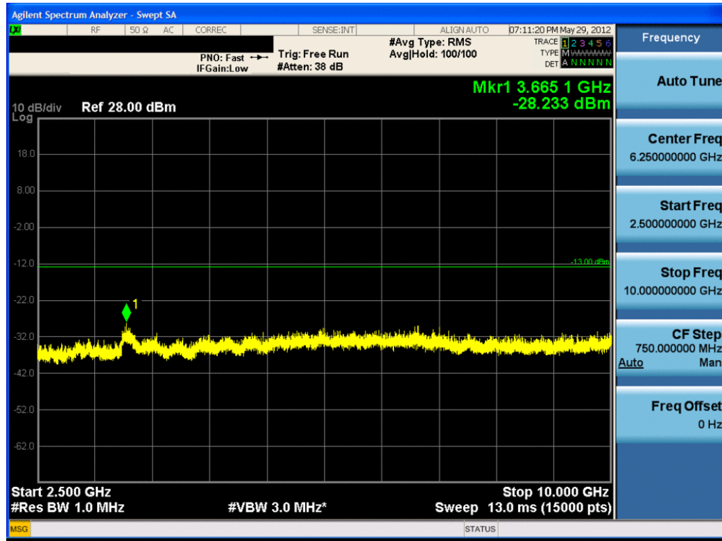
Plot 7-25. Conducted Spurious Plot (Cellular EvDO Mode – Ch. 1013)
