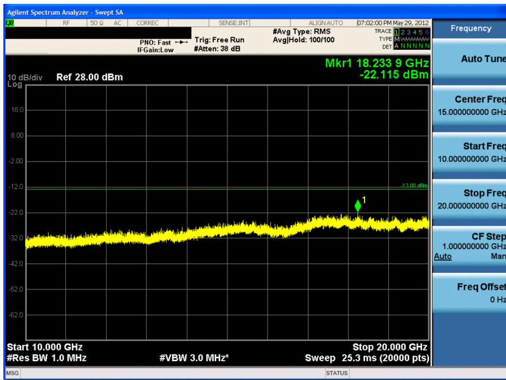
Plot 7-36. Conducted Spurious Plot (PCS EvDO Mode – Ch. 25)
