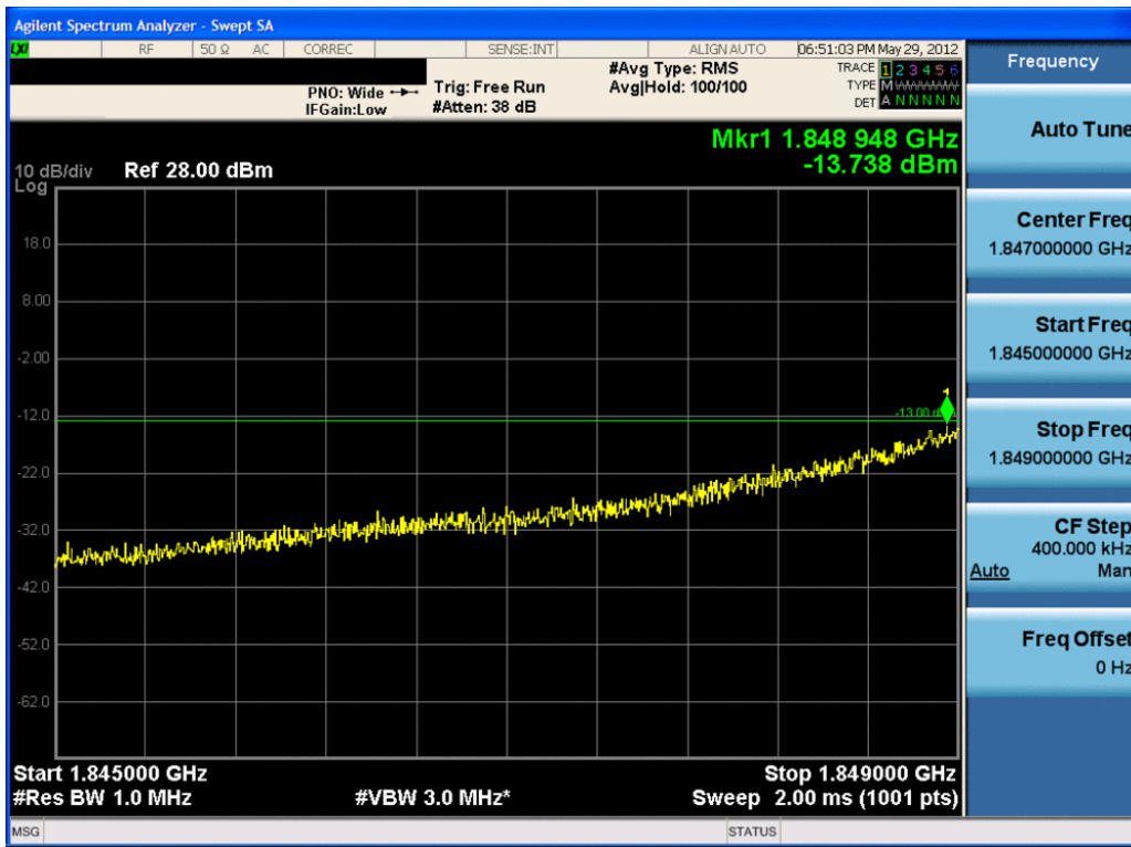
Plot 7-38. 4MHz Span Plot (PCS EvDO Mode – Ch. 25)
