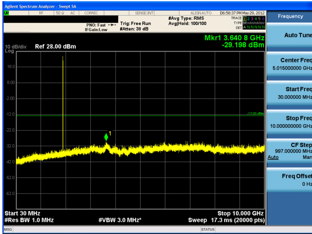
Plot 7-43. Conducted Spurious Plot (PCS EvDO Mode – Ch. 1175)
