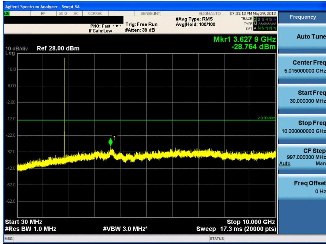
Plot 7-35. Conducted Spurious Plot (PCS EvDO Mode – Ch. 25)
