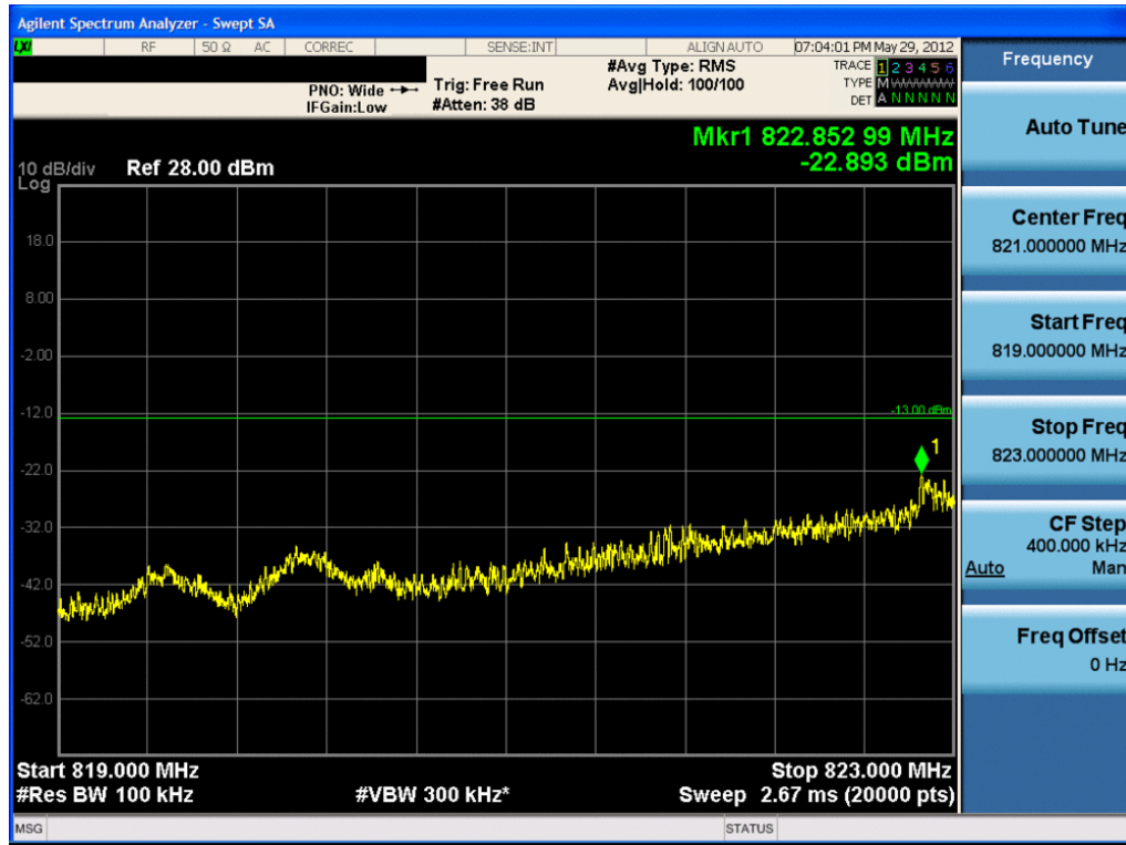
Plot 7-27. 4MHz Span Plot (Cellular EvDO Mode – Ch. 1013)
