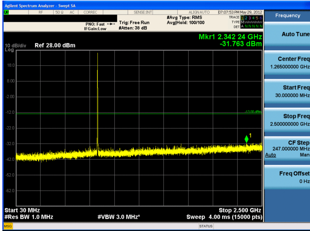
Plot 7-31. Conducted Spurious Plot (Cellular EvDO Mode – Ch. 777)
