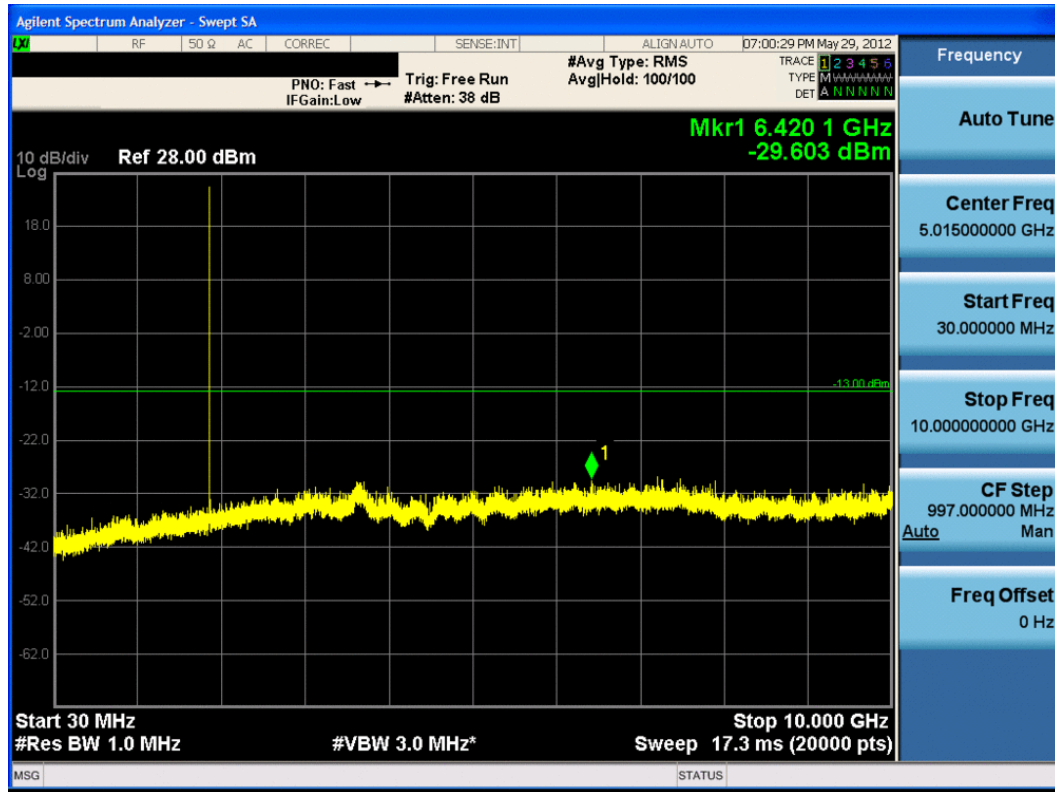
Plot 7-39. Conducted Spurious Plot (PCS EvDO Mode – Ch. 600)
