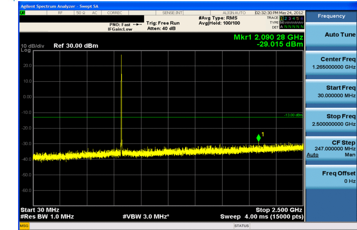
Plot 7-5. Conducted Spurious Plot (Cellular CDMA Mode – Ch. 384)
