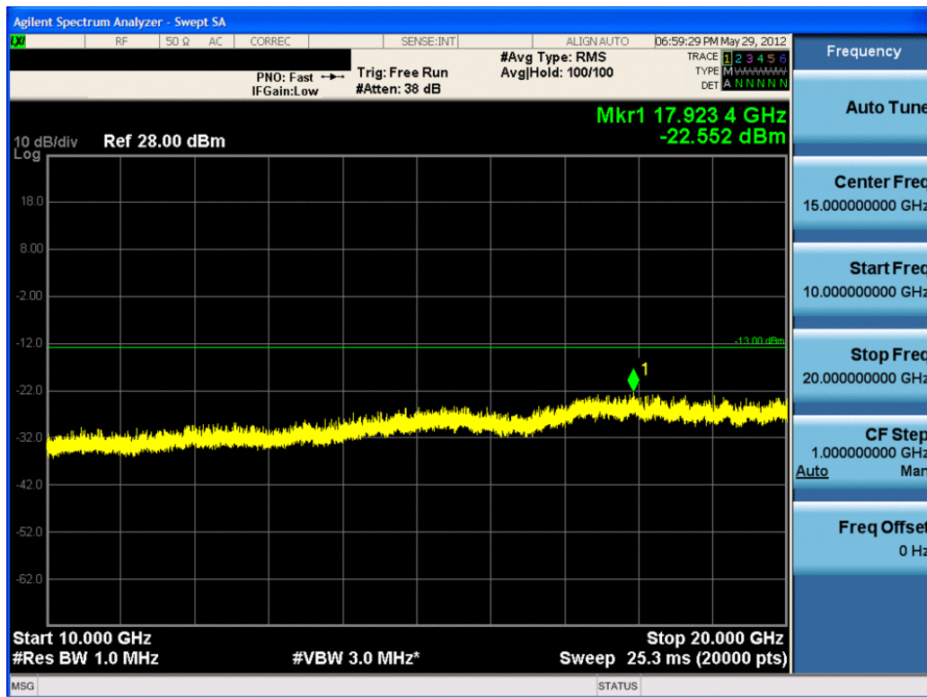
Plot 7-44. Conducted Spurious Plot (PCS EvDO Mode – Ch. 1175)
