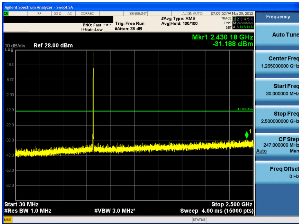
Plot 7-28. Conducted Spurious Plot (Cellular EvDO Mode – Ch. 384)
