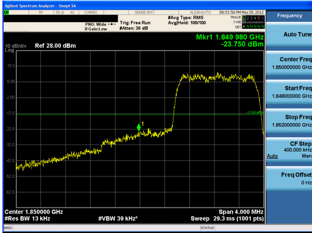
Plot 7-37. Band Edge Plot (PCS EvDO Mode – Ch. 25)
