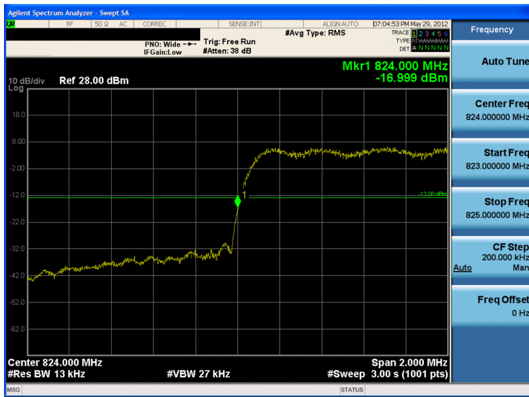
Plot 7-26. Band Edge Plot (Cellular EvDO Mode – Ch. 1013)
