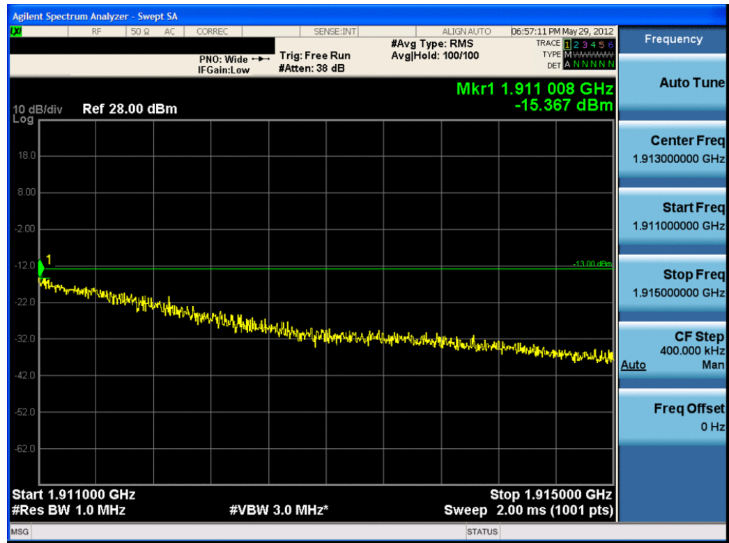
Plot 7-46. 4MHz Span Plot (PCS EvDO Mode – Ch. 1175)
