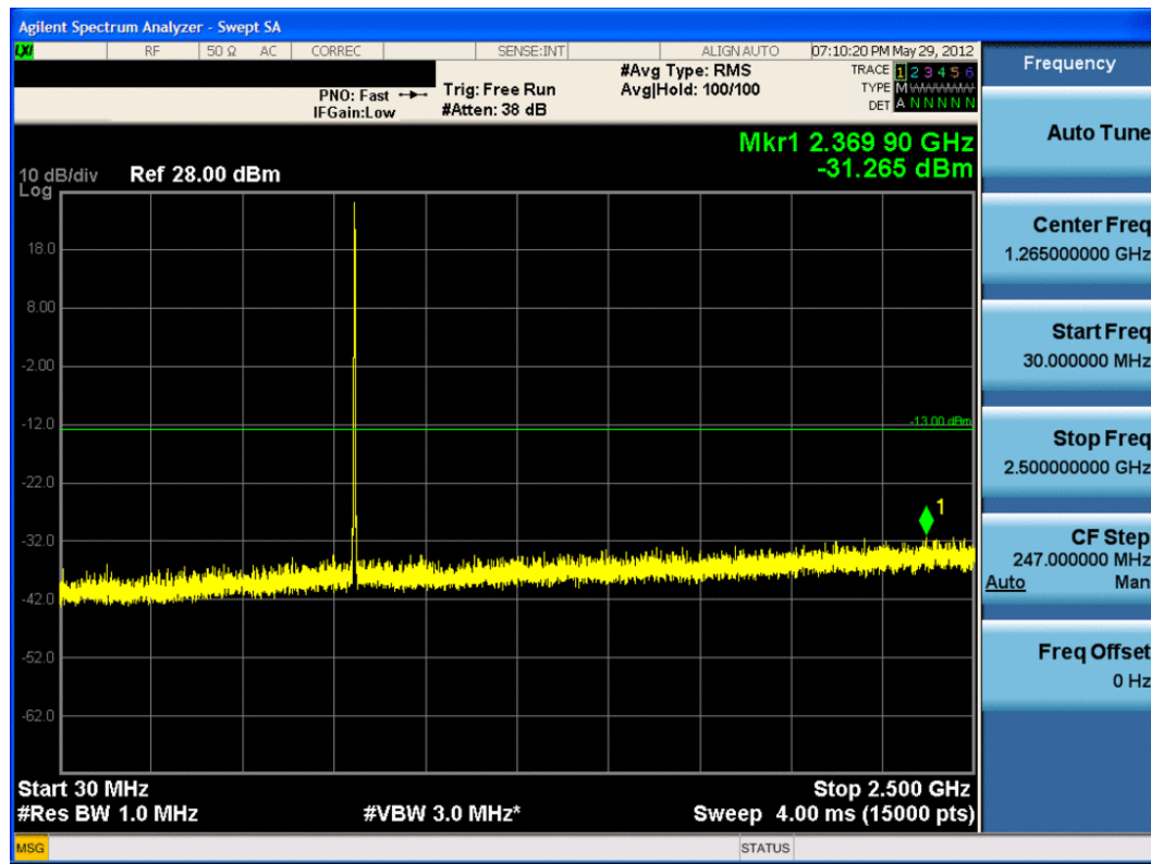
Plot 7-24. Conducted Spurious Plot (Cellular EvDO Mode – Ch. 1013)
