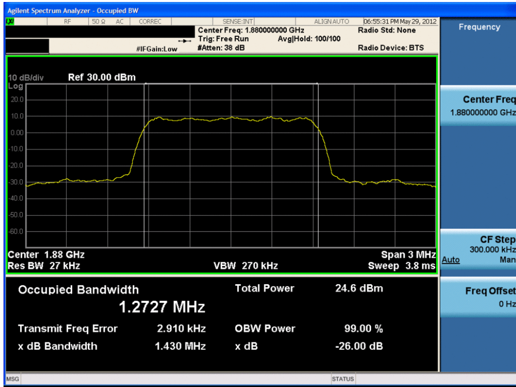
Plot 7-41. Occupied Bandwidth Plot (PCS EvDO Mode – Ch. 600)
