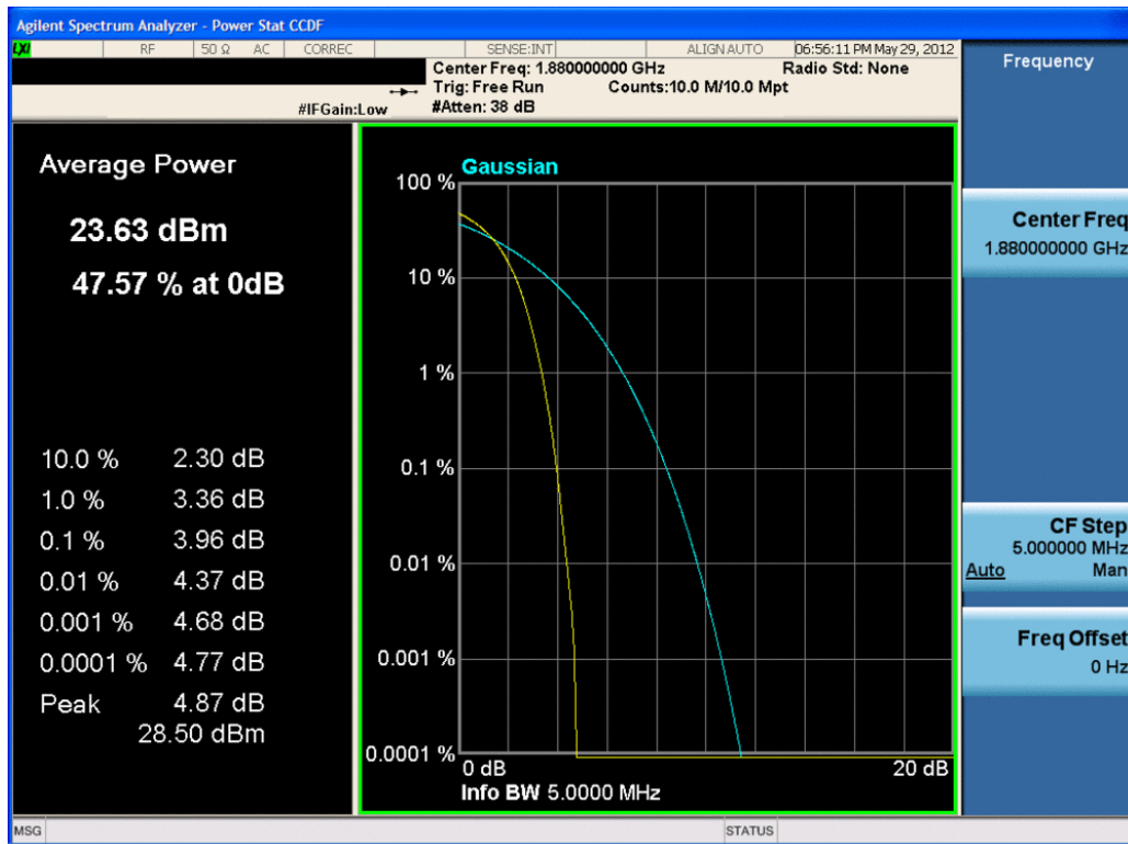
Plot 7-42. Peak-Average Ratio Plot (PCS EvDO Mode – Ch. 600)
