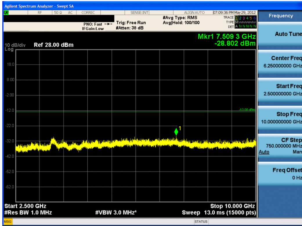
Plot 7-29. Conducted Spurious Plot (Cellular EvDO Mode – Ch. 384)
