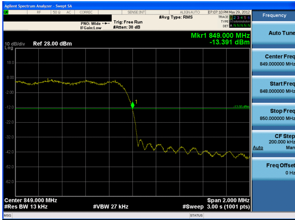
Plot 7-33. Band Edge Plot (Cellular EvDO Mode – Ch. 777)
