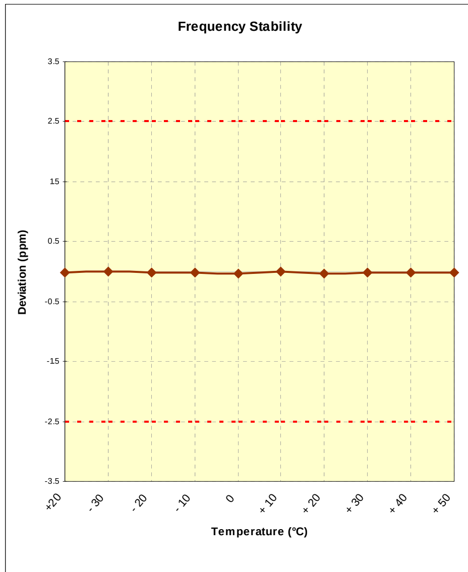
Figure 6-3. Frequency Stability Graph (Cellular EvDO Mode – Ch. 384)
