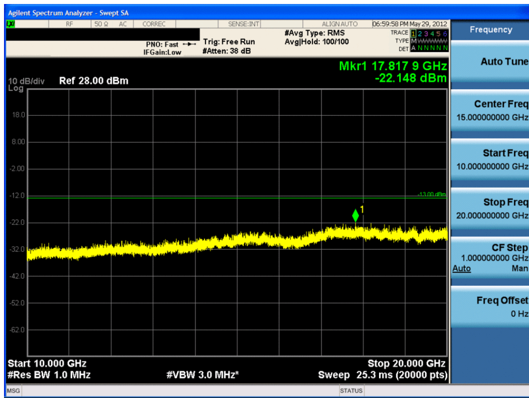
Plot 7-40. Conducted Spurious Plot (PCS EvDO Mode – Ch. 600)
