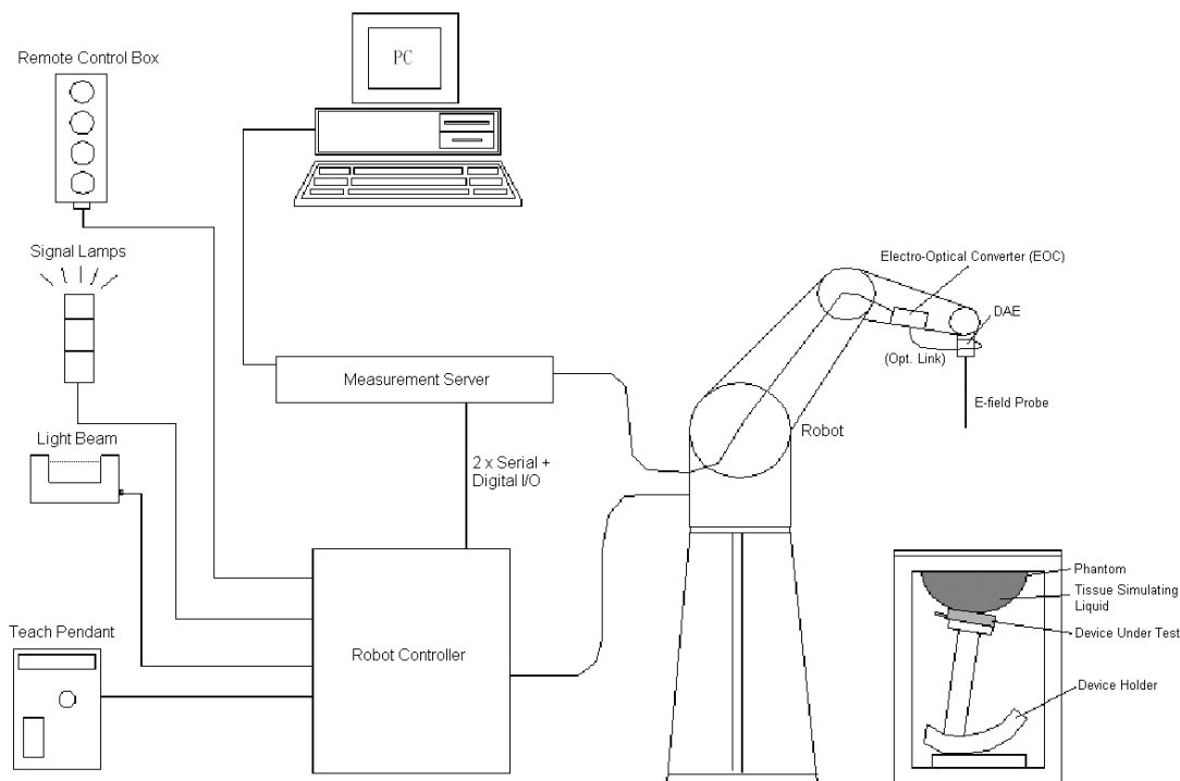
Fig 5.1 SPEAG DASY System Configurations
