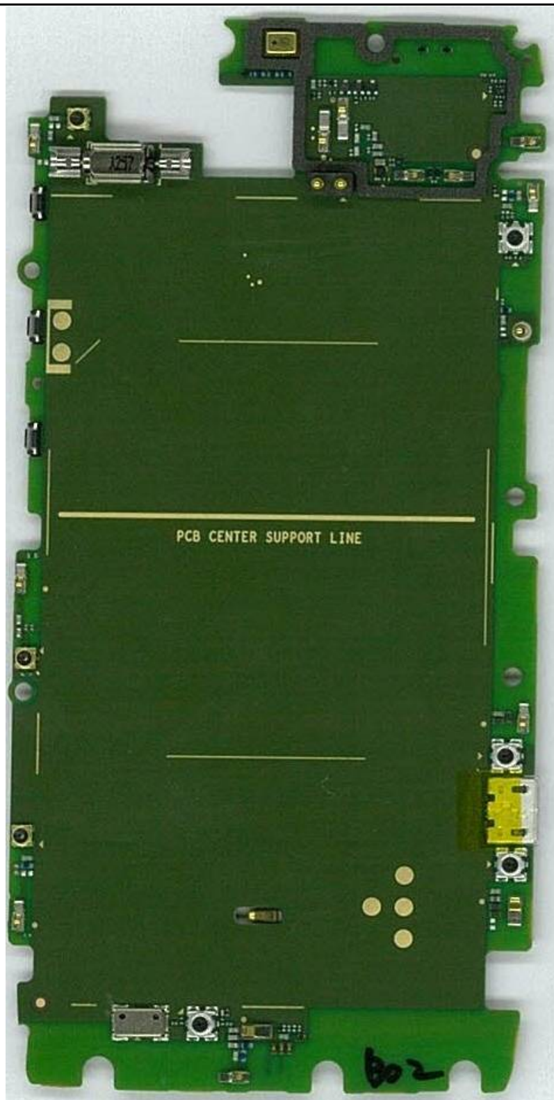
Photograph 9-3: Rear side view of the device's PC Board.
