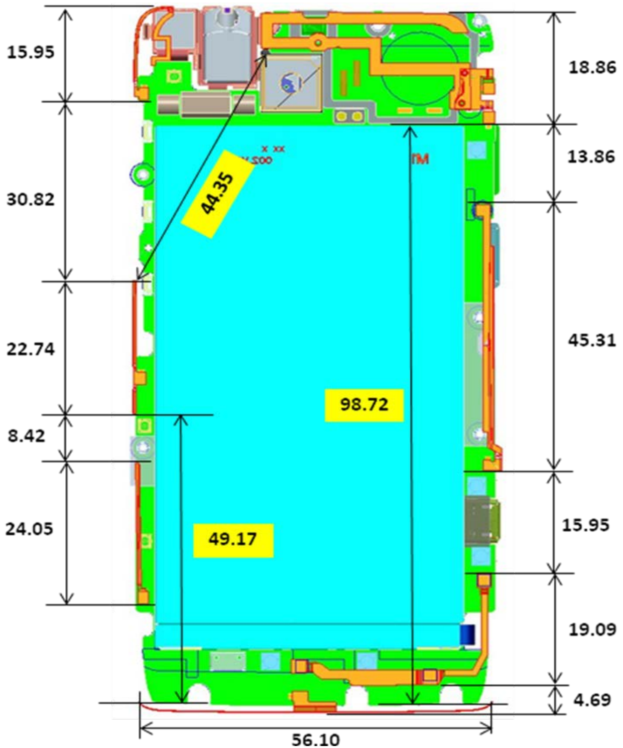
Photograph 9-7: Distances between Key Antennas.
