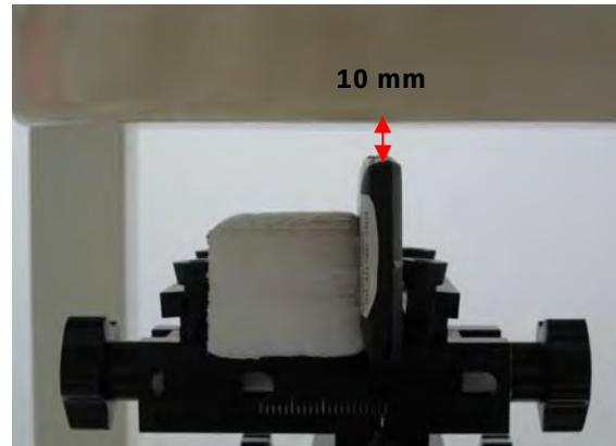
Fig.13 EUT Left to flat phantom
