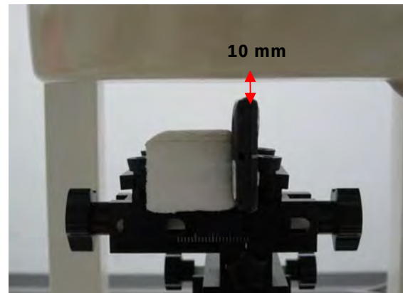
Fig.12 EUT Right to flat phantom
