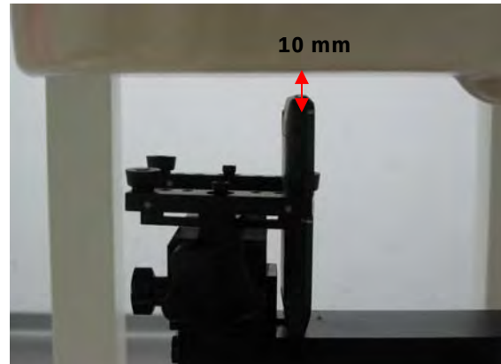
Fig.10 EUT Top to flat phantom
