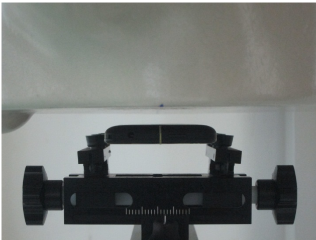
Back of the EUT with Phantom 1.0 cm Gap
