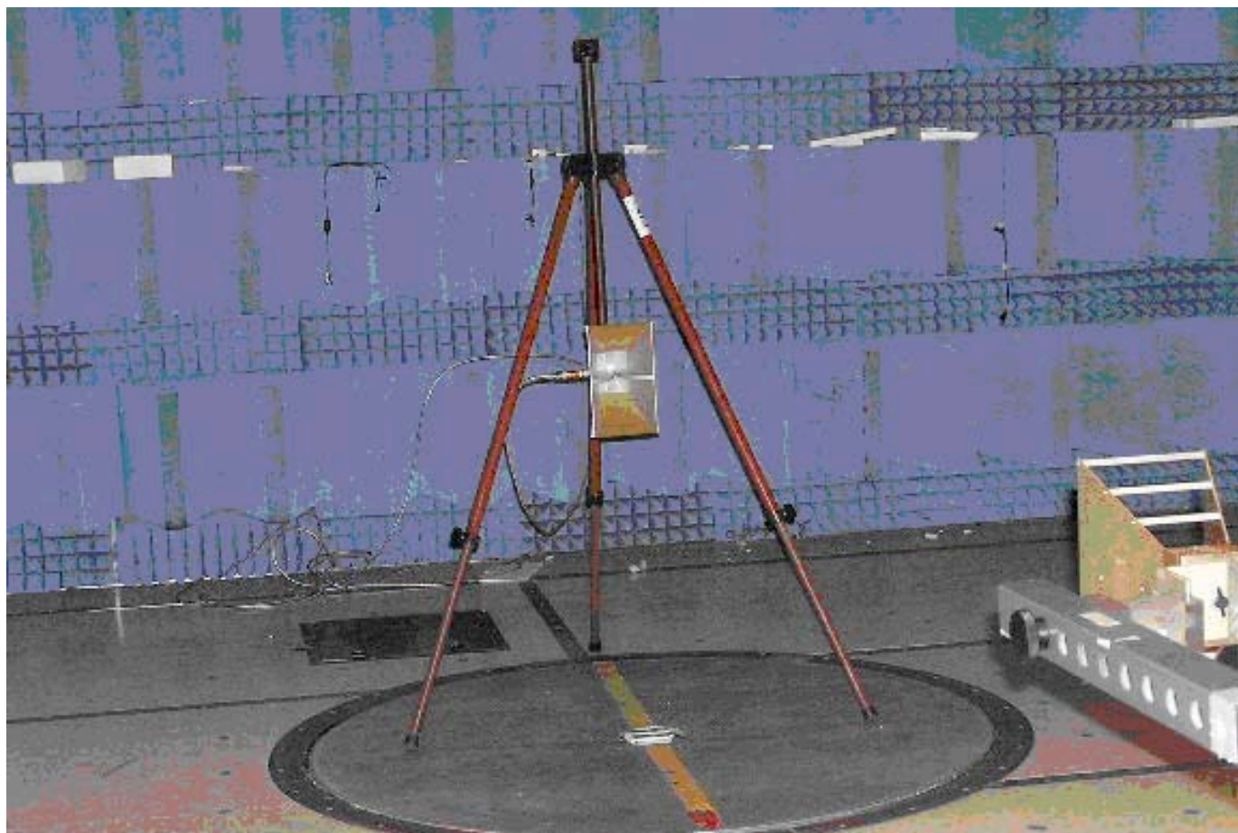
Figure 7c1-2: Antenna - Substitution.
