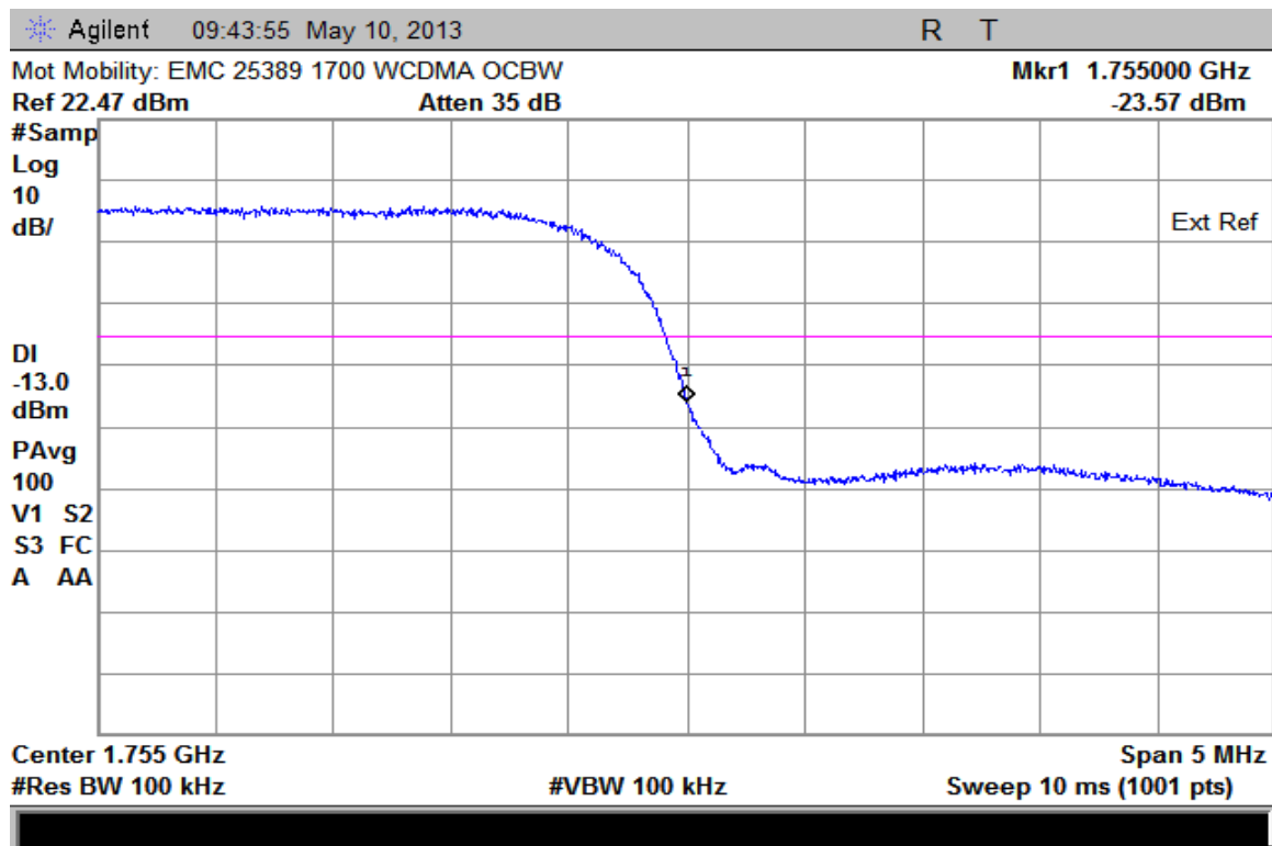
WCDMA 1700 – Upper Band Edge – Channel 1513 (1752.6 MHz)
