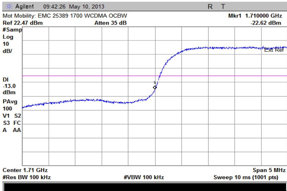
WCDMA 1700 – Lower Band Edge – Channel 1312 (1712.4 MHz)
