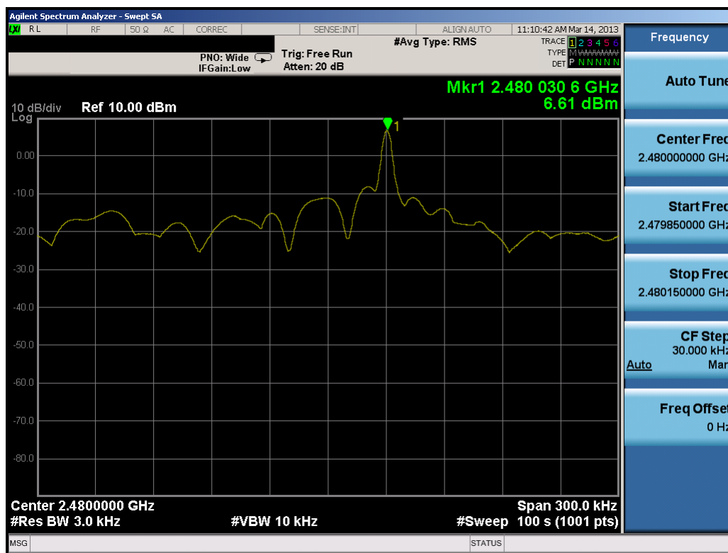
Plot 6-6. Power Spectral Density Plot (Bluetooth (LE) – Ch. 39)
