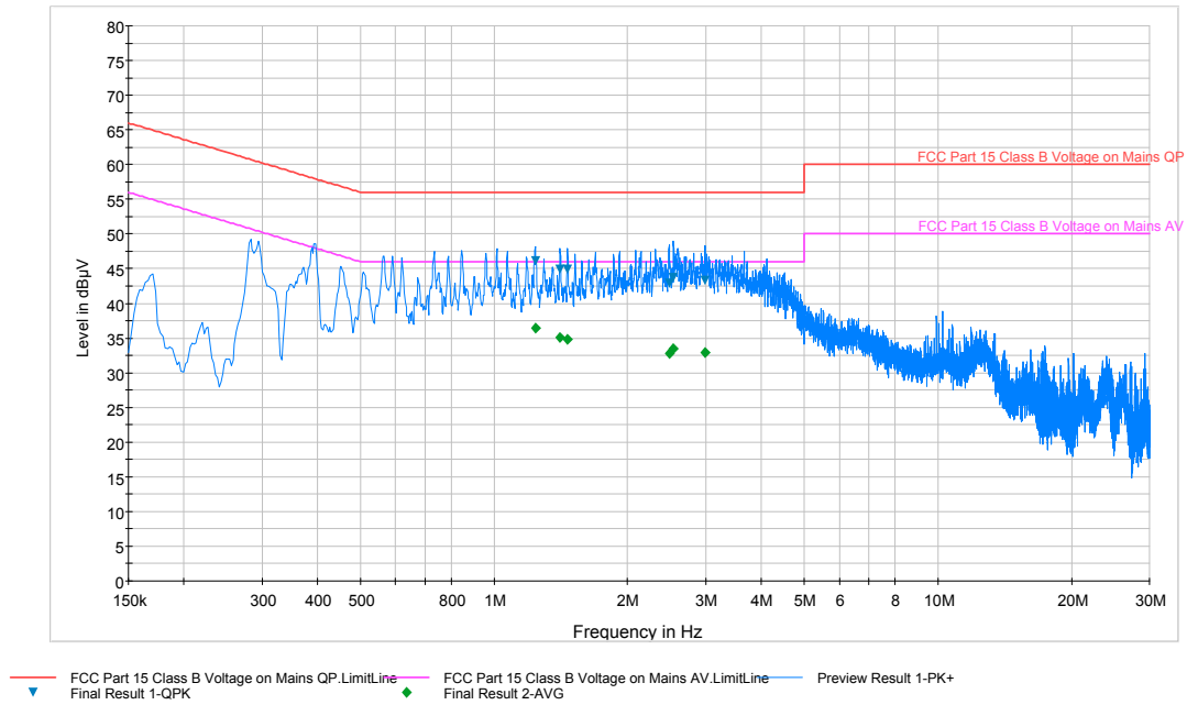
Plot 6-78. Line Conducted Plot with 802.11a (N)
