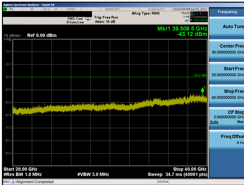
Plot 6-56. Conducted Spurious Plot (802.11a – Ch. 149)
