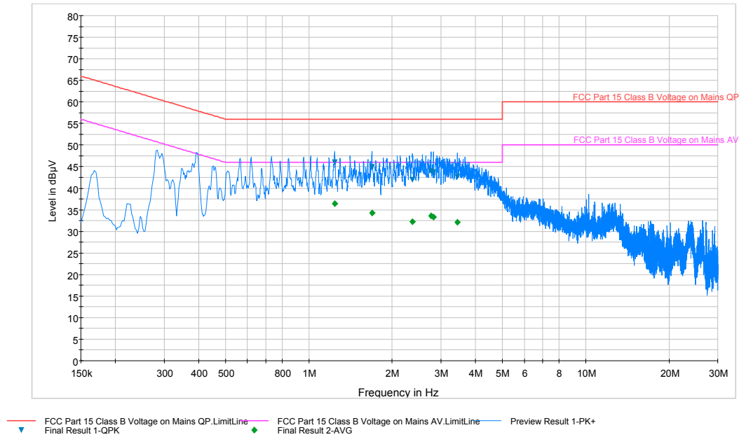
Plot 6-76. Line Conducted Plot with 802.11b (N)
