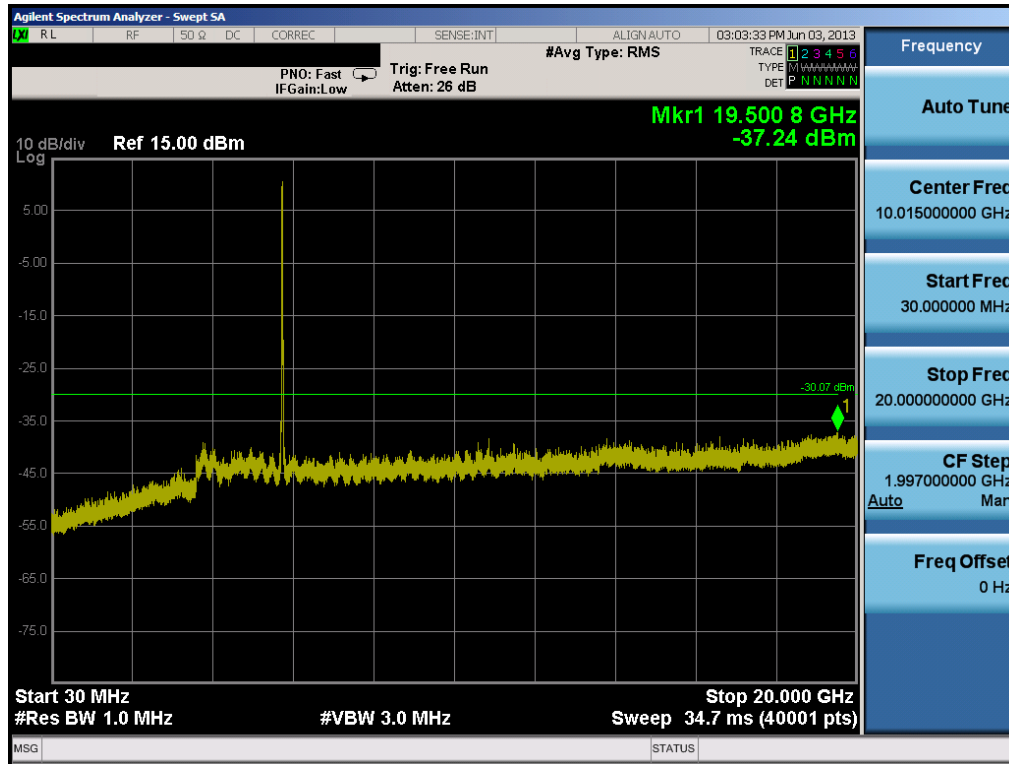
Plot 6-55. Conducted Spurious Plot (802.11a – Ch. 149)
