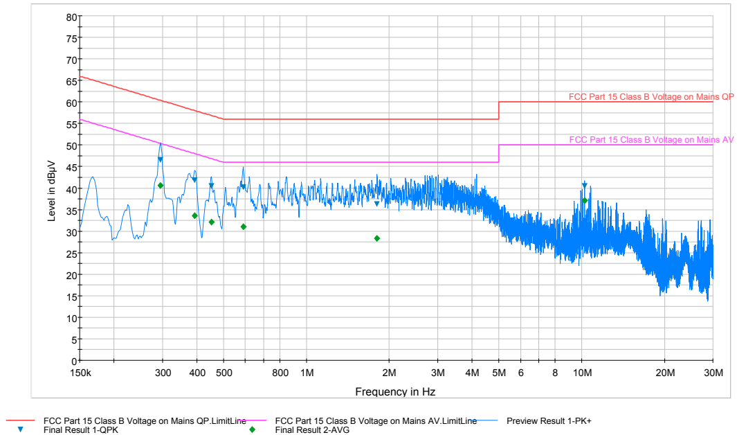
Plot 6-75. Line Conducted Plot with 802.11b (L1)
