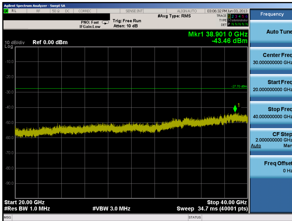
Plot 6-58. Conducted Spurious Plot (802.11a – Ch. 157)
