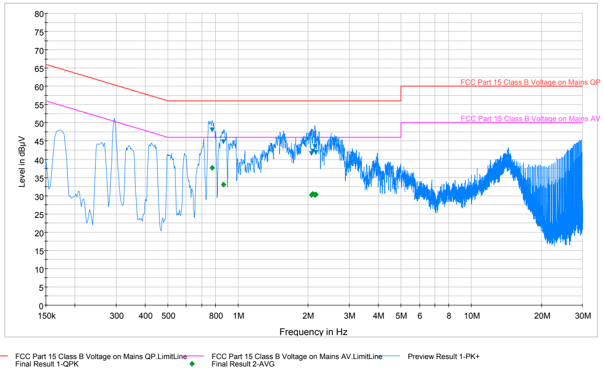
Plot 6-80. Line Conducted Plot with 802.11b (N w/ WCP)
