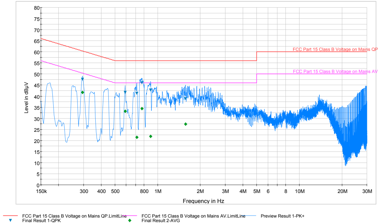
Plot 6-79. Line Conducted Plot with 802.11b (L1 w/ WCP)
