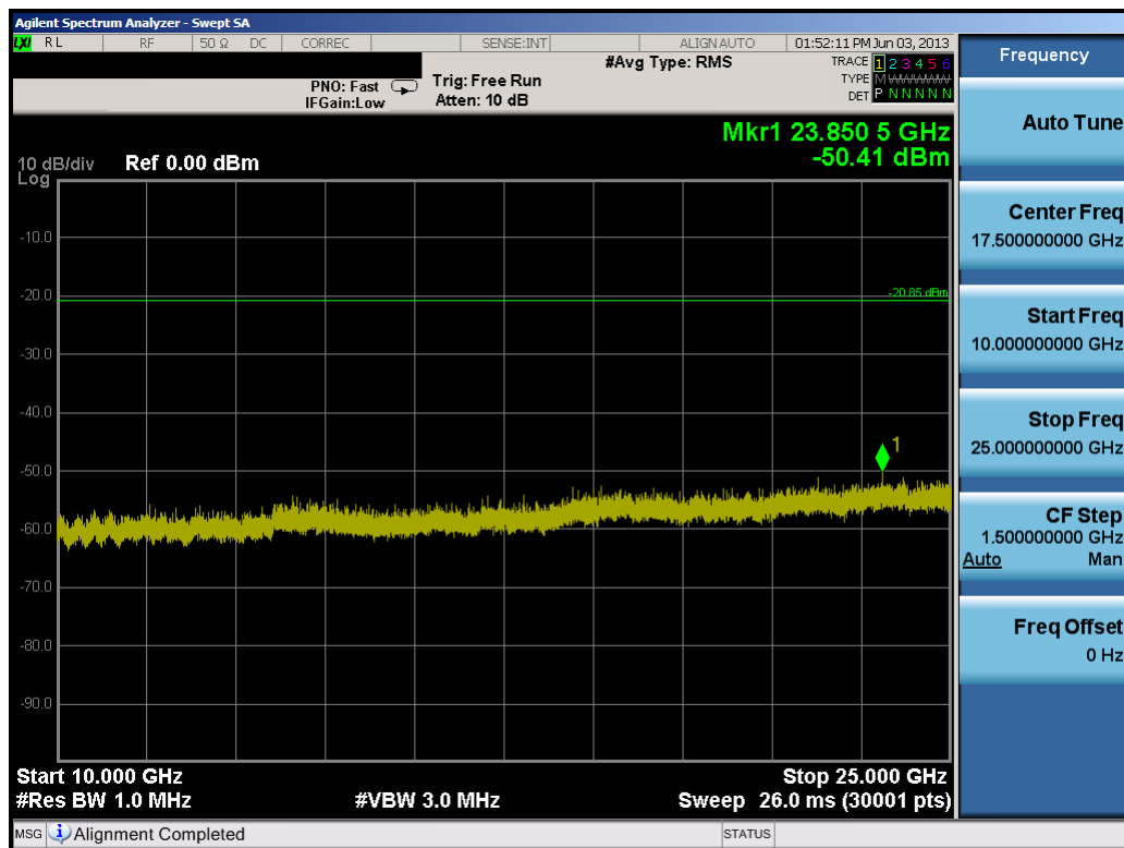
Plot 6-54. Conducted Spurious Plot (802.11b – Ch. 11)
