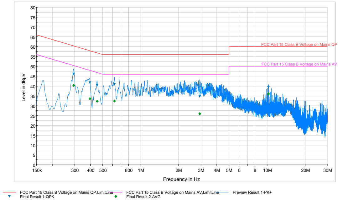
Plot 6-77. Line Conducted Plot with 802.11a (L1)
