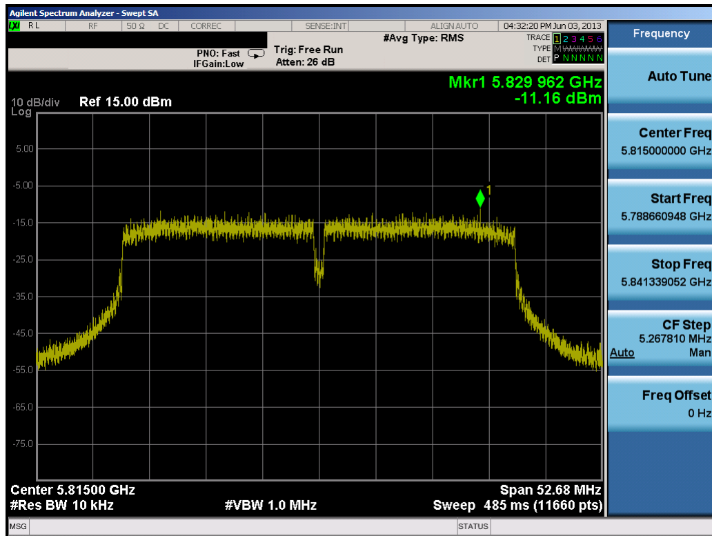
Plot 6-36. Power Spectral Density Plot (40MHz BW 802.11n (5.8GHz) – Ch. 163)
