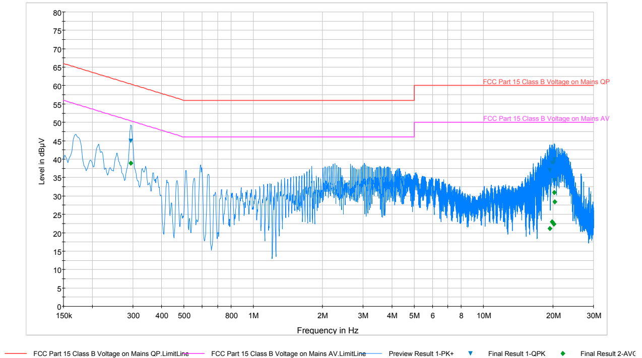
Plot 6-46. Line-Conducted Test Plot (L1)
