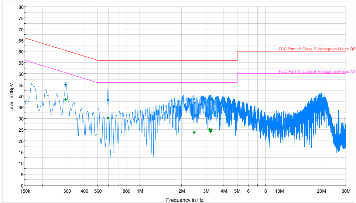
Plot 6-47. Line-Conducted Test Plot (N)
