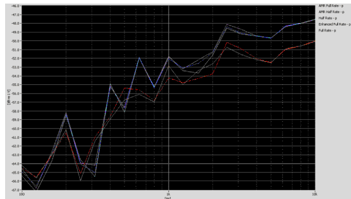
Figure 5-12 Vocoder Analysis for GSM ABM Noise
