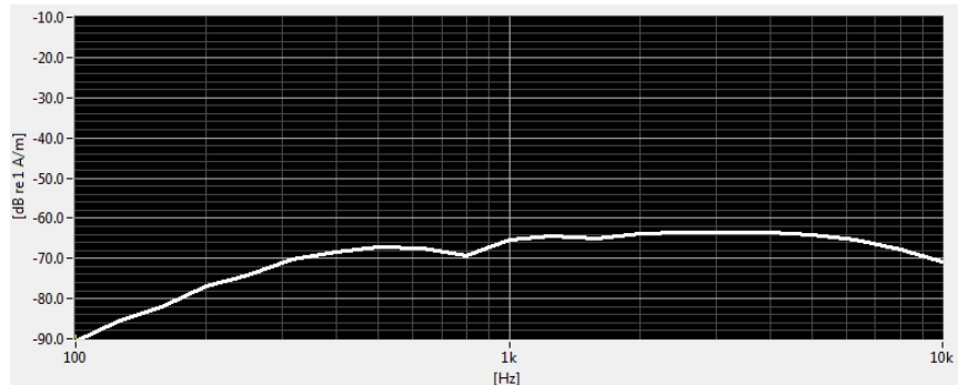
Figure 7-2 Worst-case ABM2 Plot for CDMA
