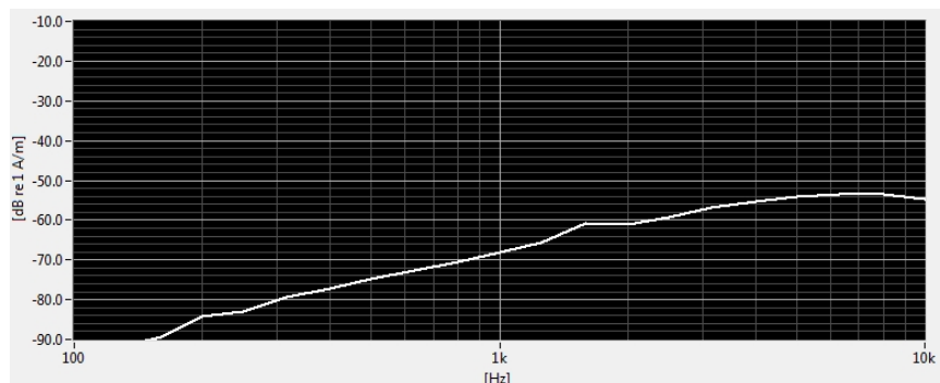
Figure 7-4 Worst-case ABM2 Plot for UMTS
