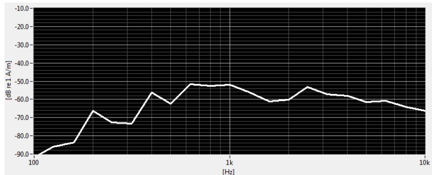
Figure 7-3 Worst-case ABM2 Plot for GSM
