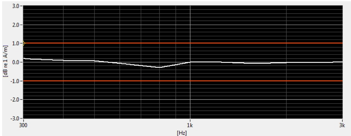
Figure 7-5 Helmholtz Coil Validation for Frequency Response
