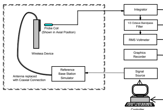
Figure 5-14 Audio Magnetic Field Test Setup
