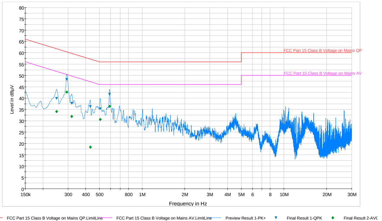
Plot 7-2. Line Conducted Plot (LN)
