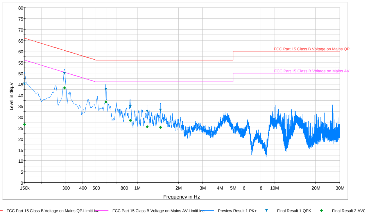
Plot 7-1. Line Conducted Plot (L1)
