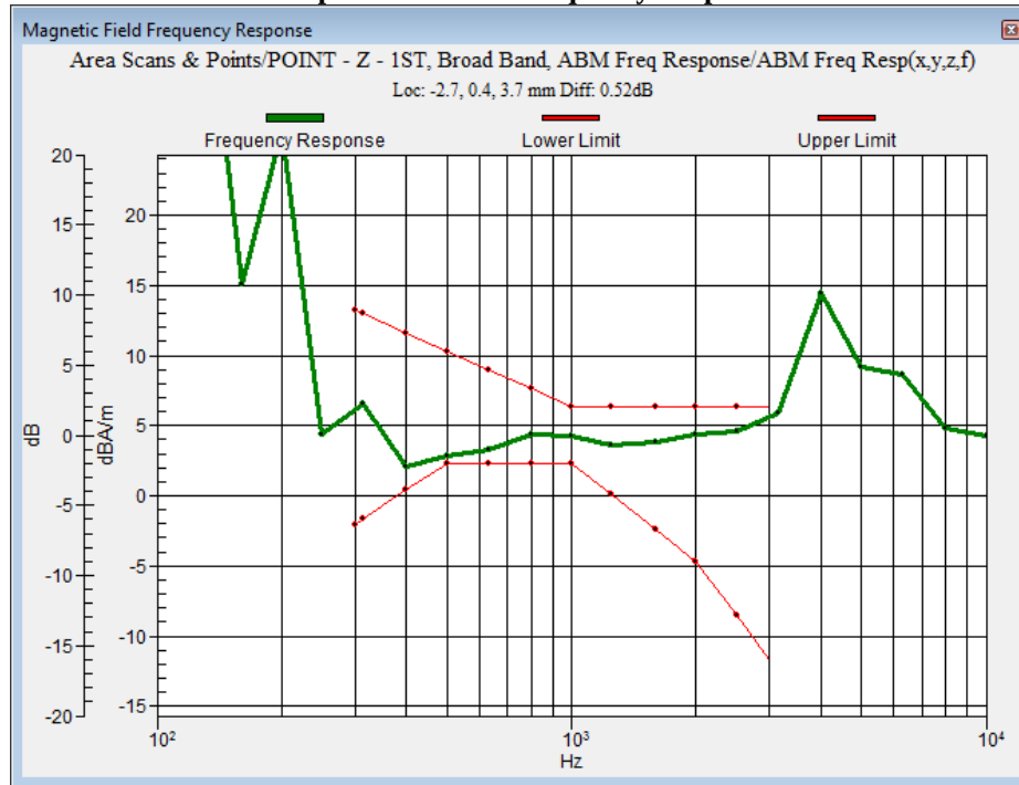
Graph 2: GSM 850 Frequency Response
