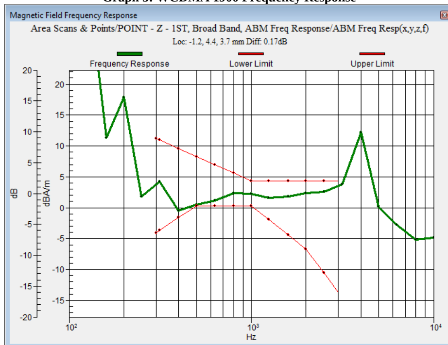
Graph 5: WCDMA 1900 Frequency Response
