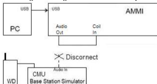
Figure 2: Signal Verification Setup
