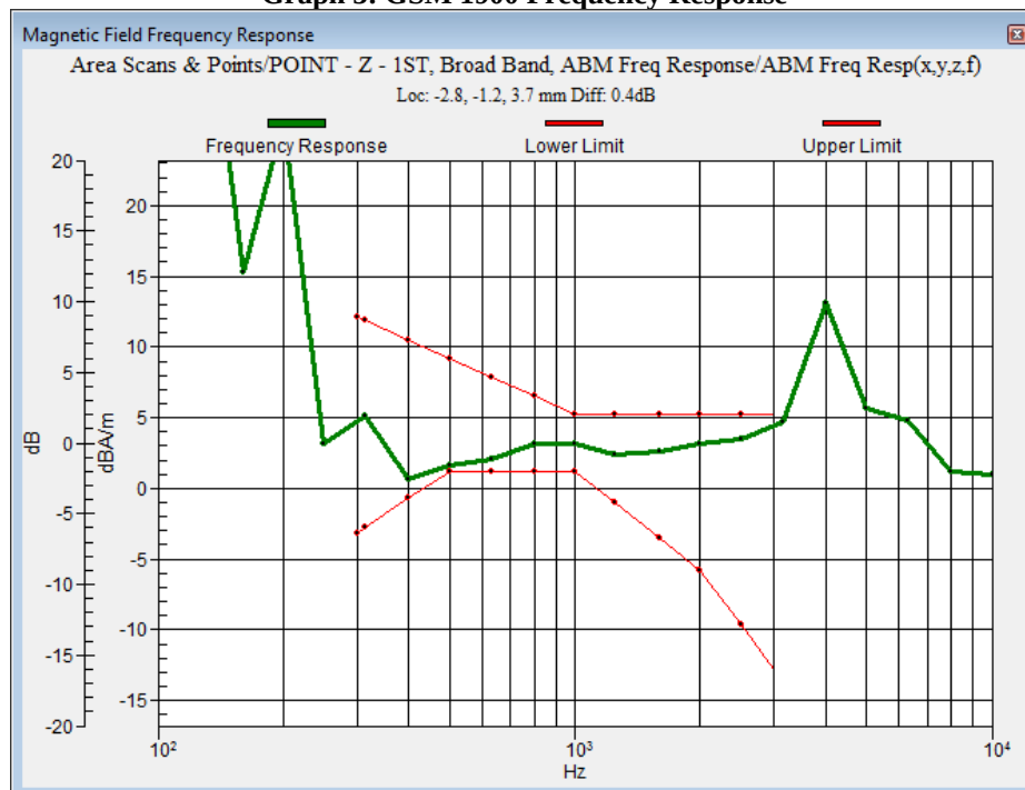
Graph 3: GSM 1900 Frequency Response
