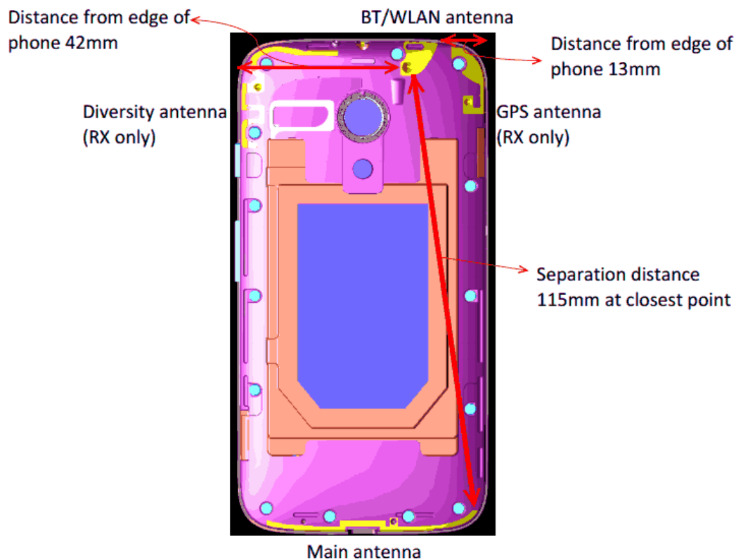
Figure 2: Antenna Separation Distances
