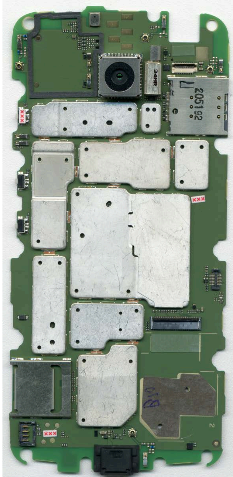
Photograph 9-1: Component side view of the device's PC Board, Shields in place.
