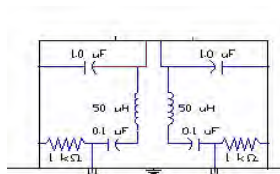
Figure 3-4. LISN Schematic Diagram
