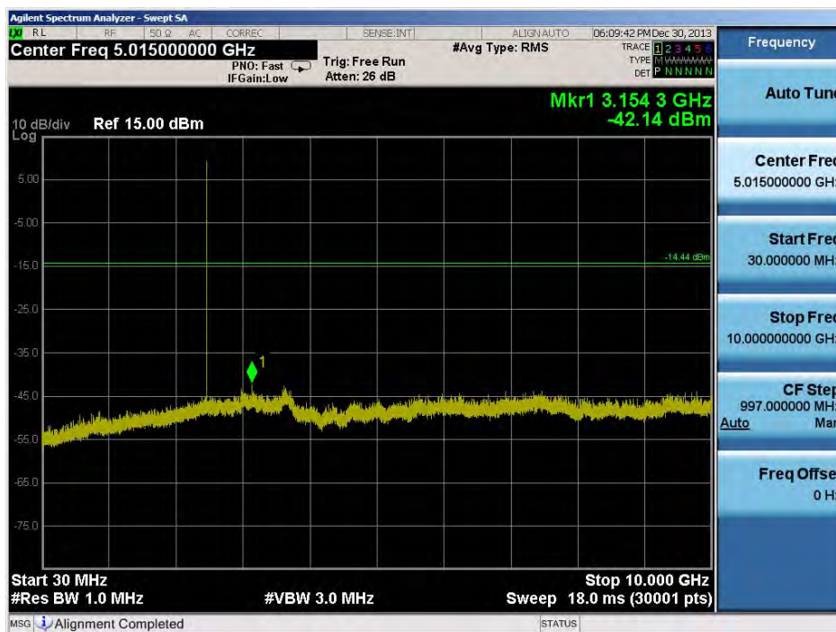
Plot 6-40. Conducted Spurious Plot (Bluetooth, 3Mbps – Ch. 78)
