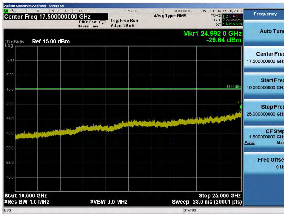
Plot 6-41. Conducted Spurious Plot (Bluetooth, 3Mbps – Ch. 78)
