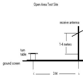
Figure 3-1. Diagram of 3-meter Test Range
