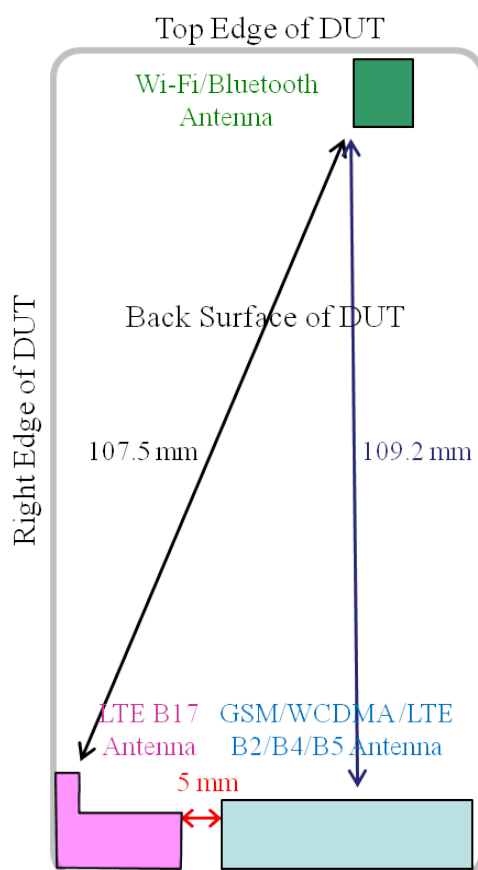
Figure 2: Antenna Separation Distances
