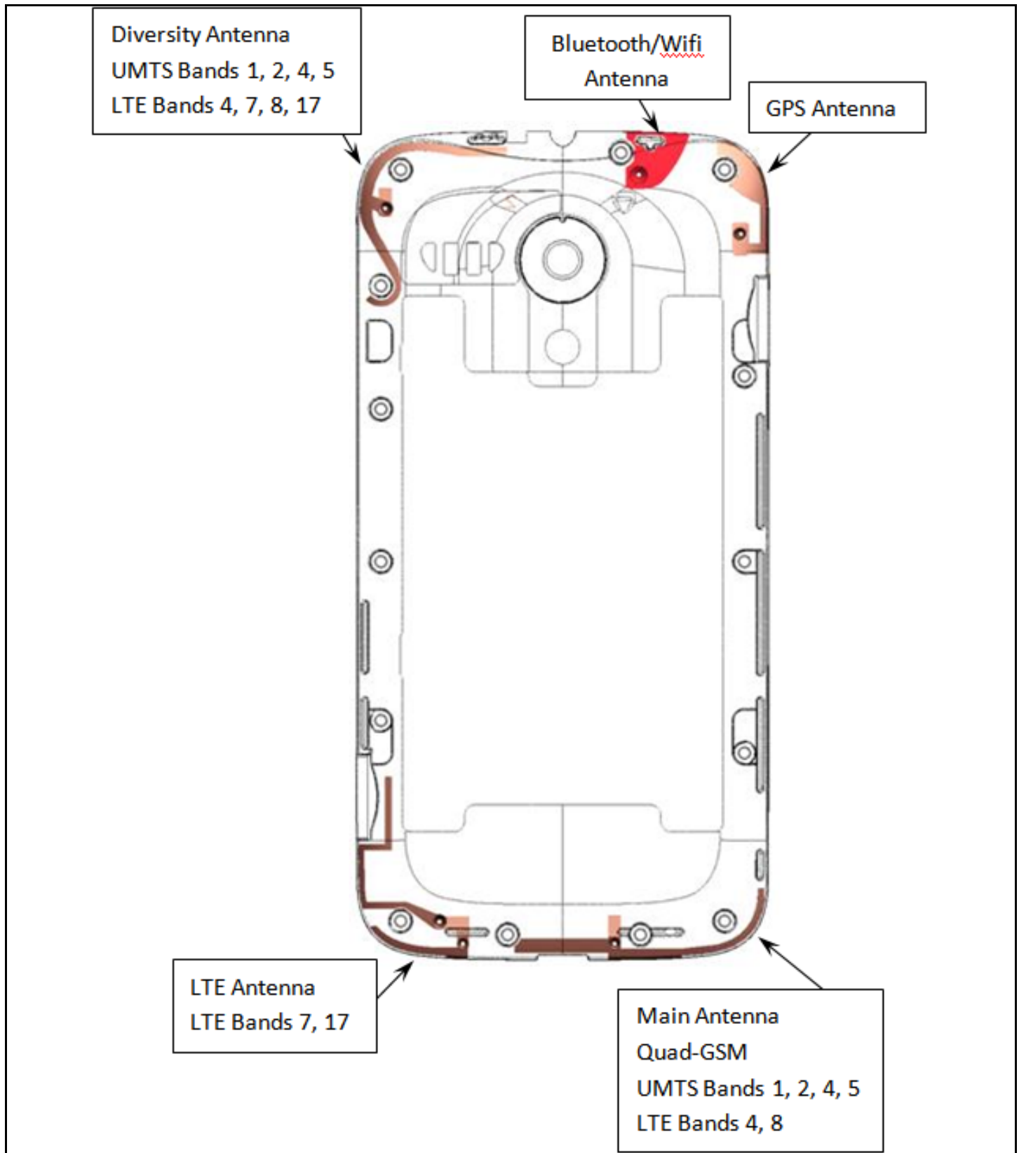
Photograph 9-4: Antenna Locations.
