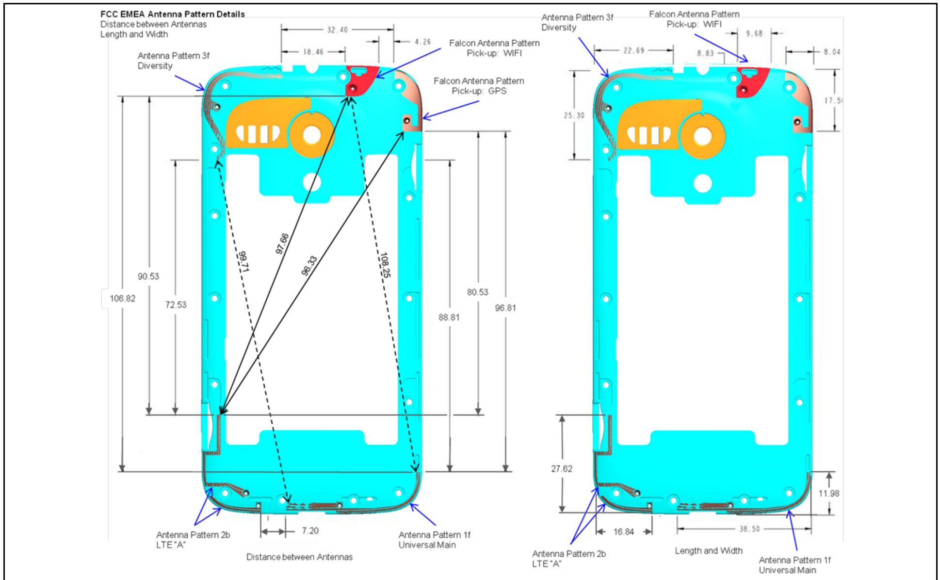
Photograph 9-5: Antenna Spacings.
