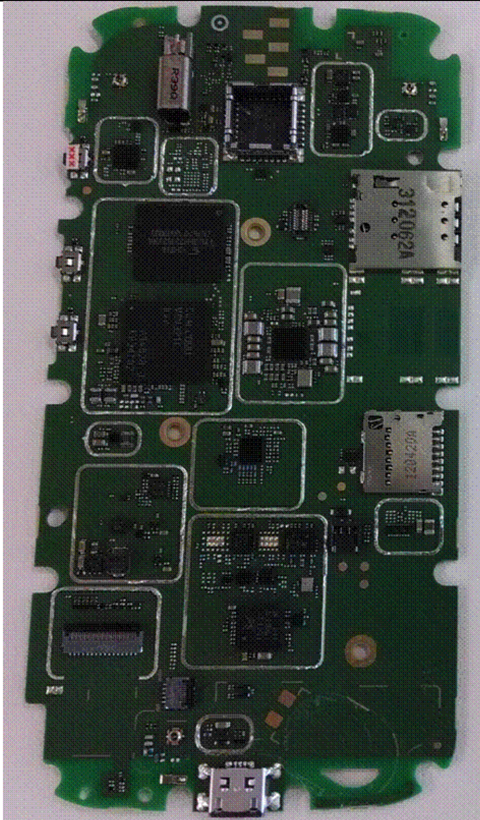
Photograph 9-2: Back side view of the device's PC Board, Shields in place.
