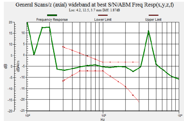
Fig 7.2 GSM1900 Ch661
