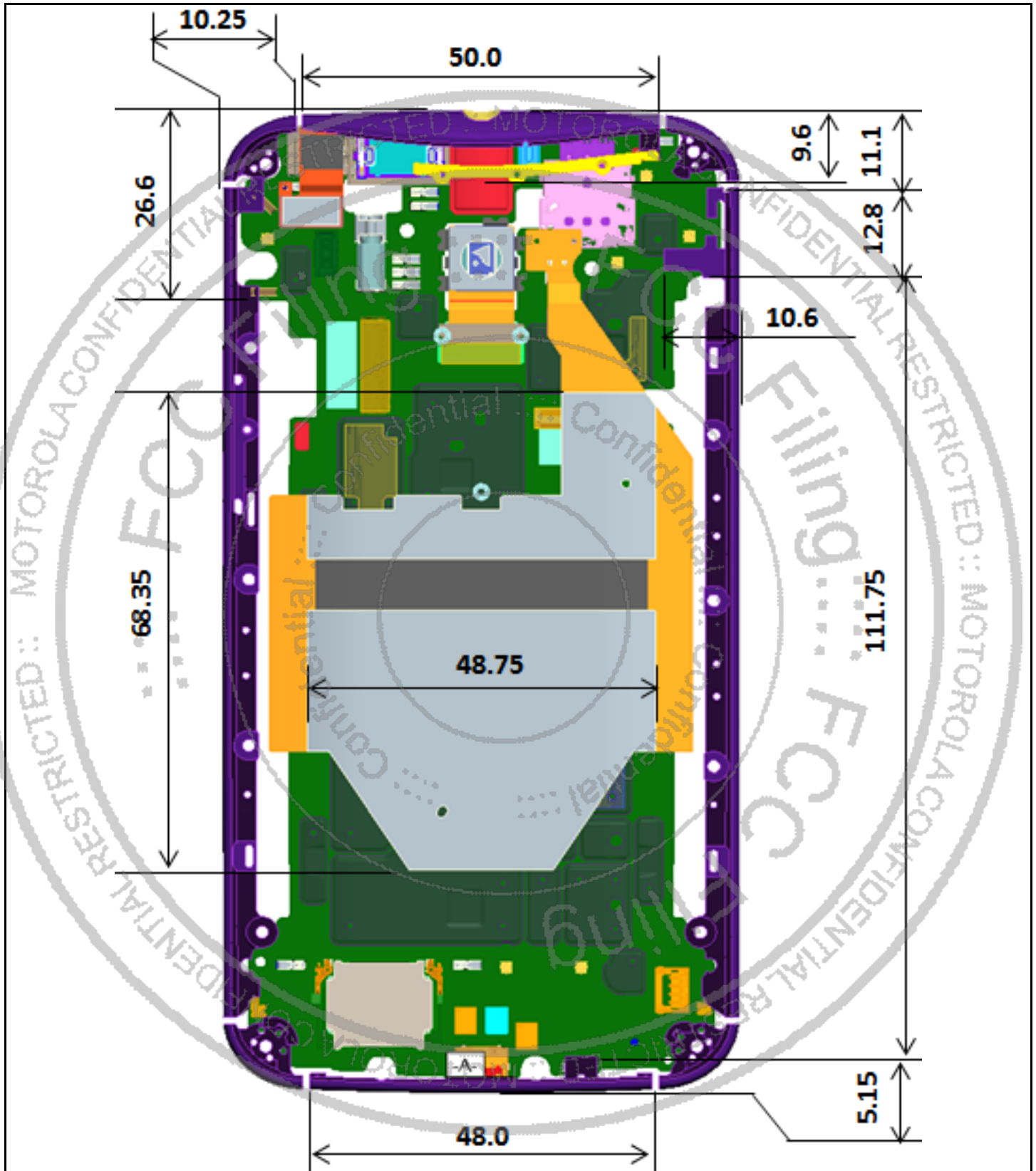
Photograph 9-5: Antenna Spacing (mm).
