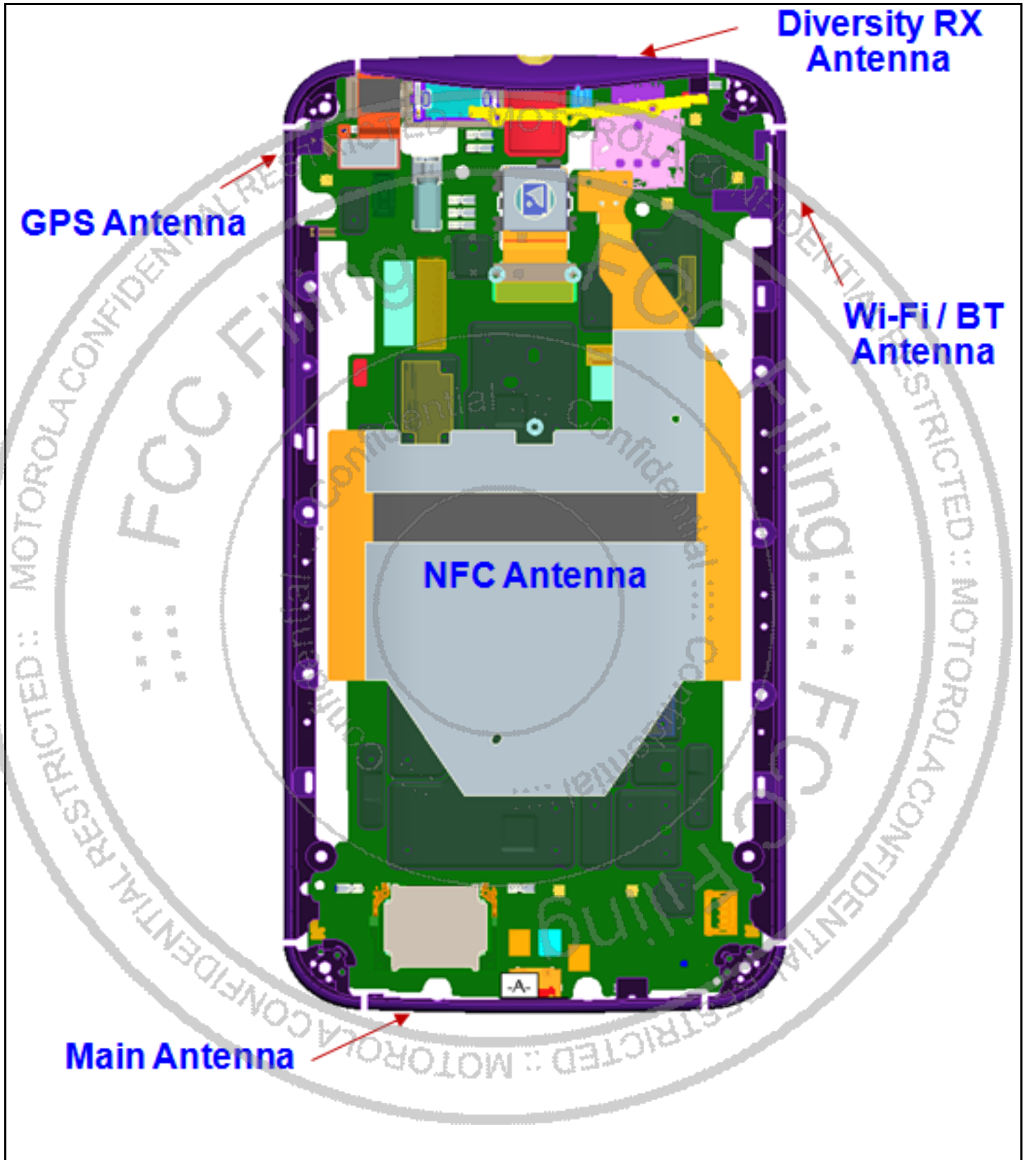
Photograph 9-4: Antenna Locations.
