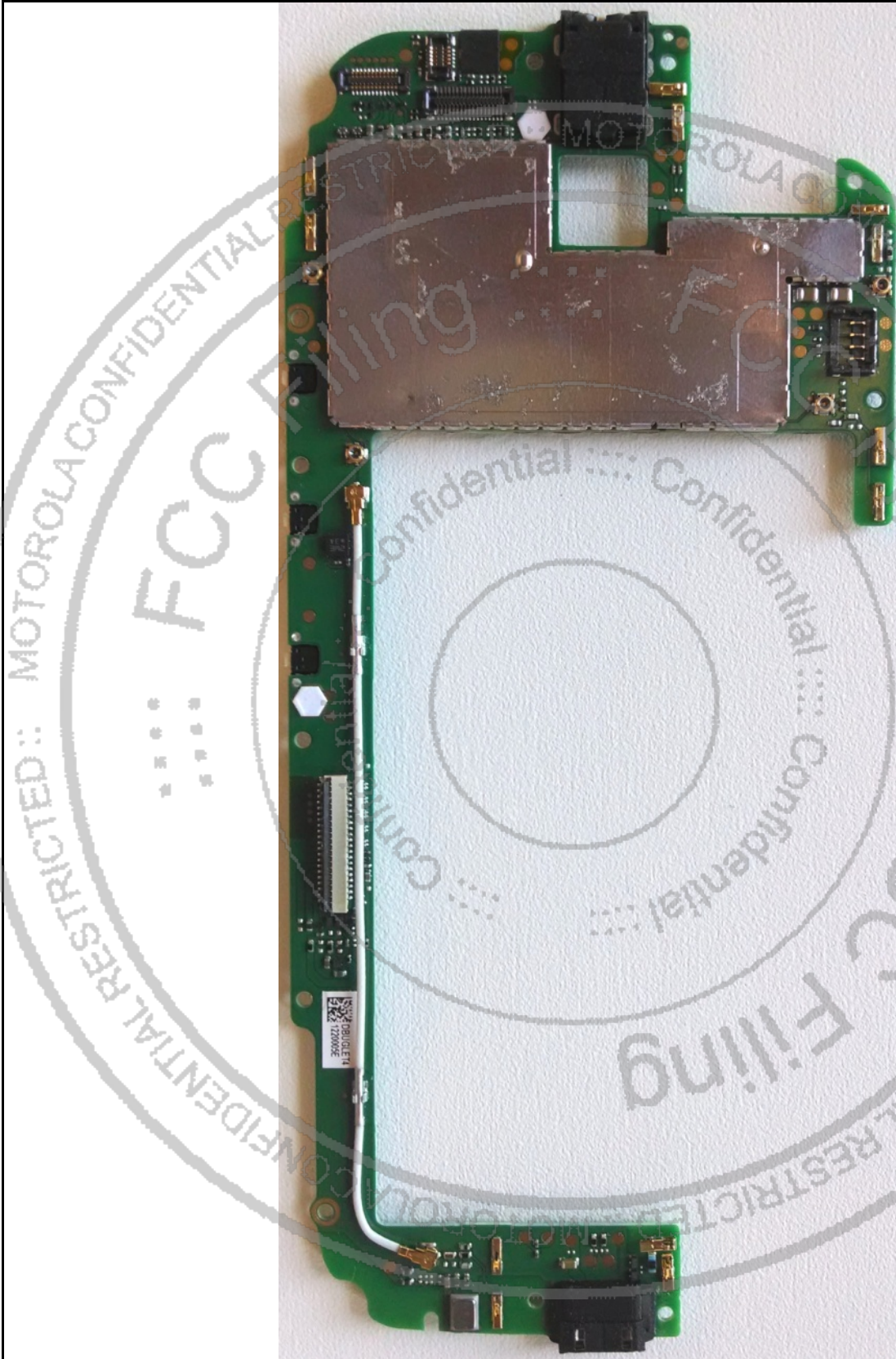
Photograph 9-2: Back side view of the device's PC Board, Shields in place.
