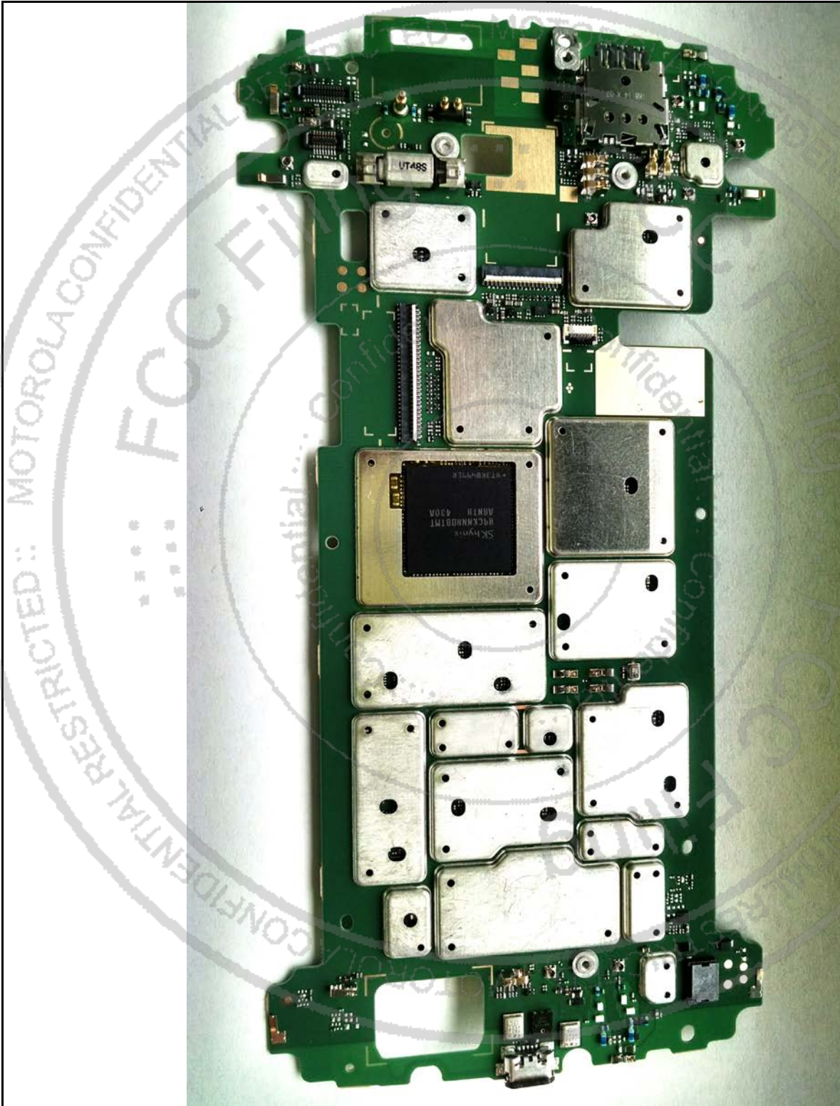
Photograph 9-1: Front side view of the device's PC Board, Shields in place.
