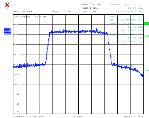
Highest Channel / 15MHz / 16QAM
