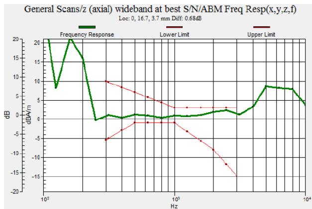
Fig. 7.7 CDMA2000 BC0 Ch384
