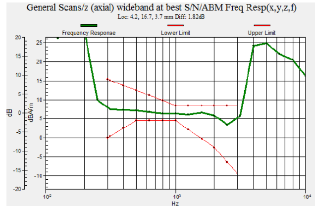
Fig 7.2 GSM1900 Ch661
