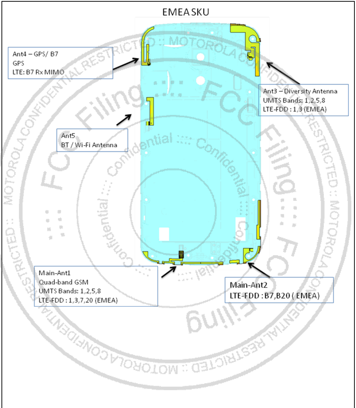
Photograph 9-5: Antenna Locations.
