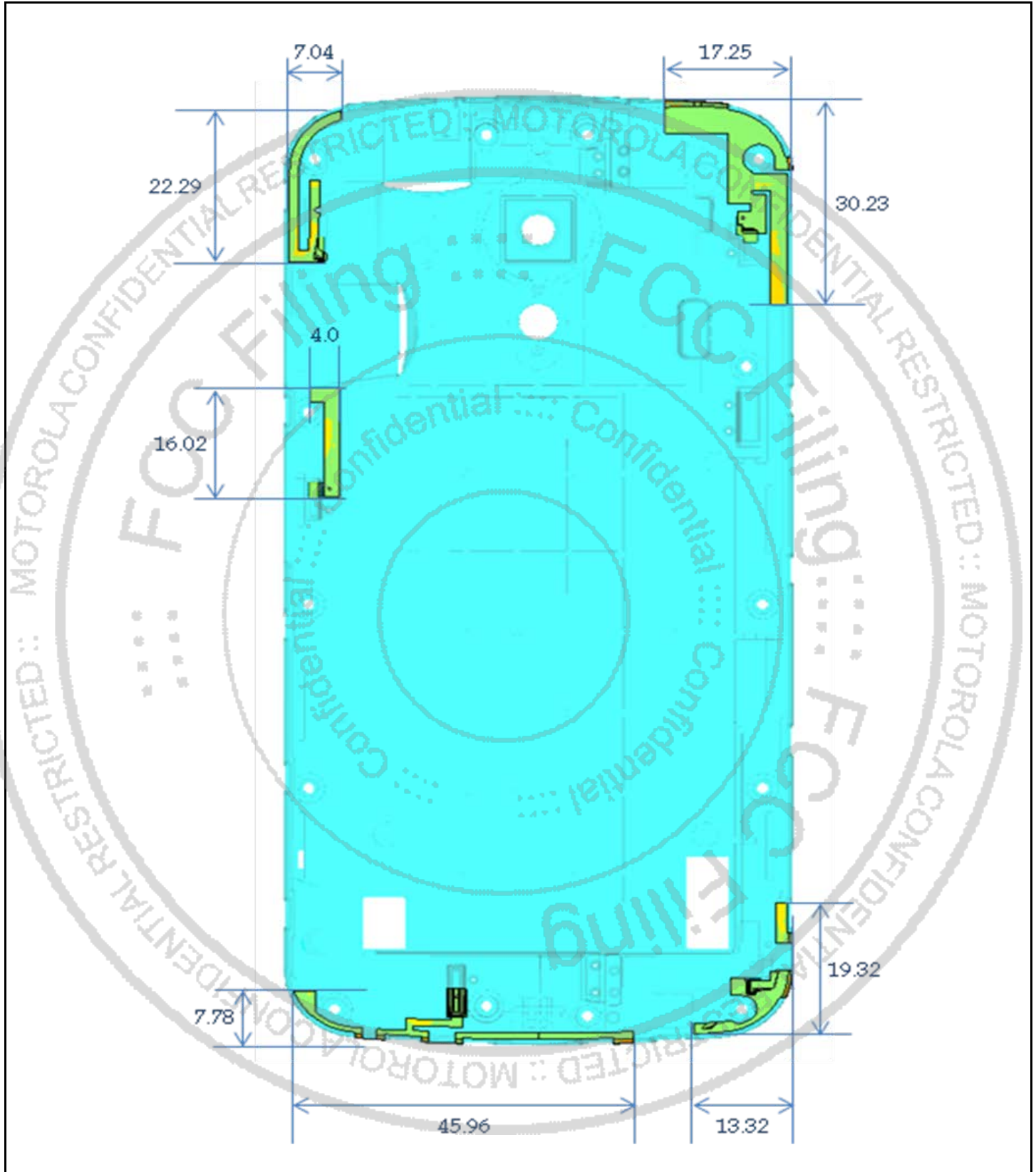
Photograph 9-6: Antenna Spacings.
