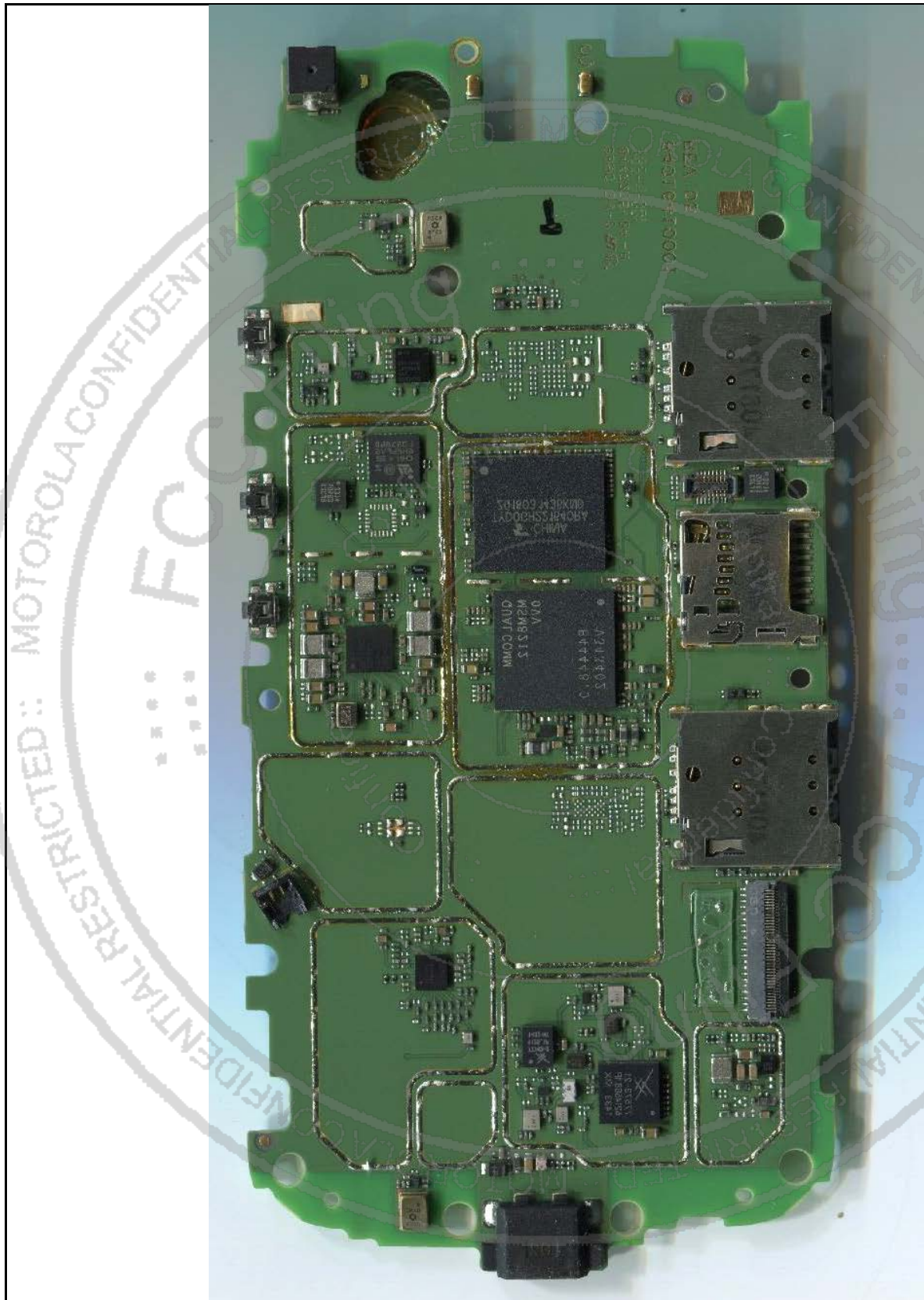
Photograph 9-3: Front side view of the device's PC Board, Shields Removed.
