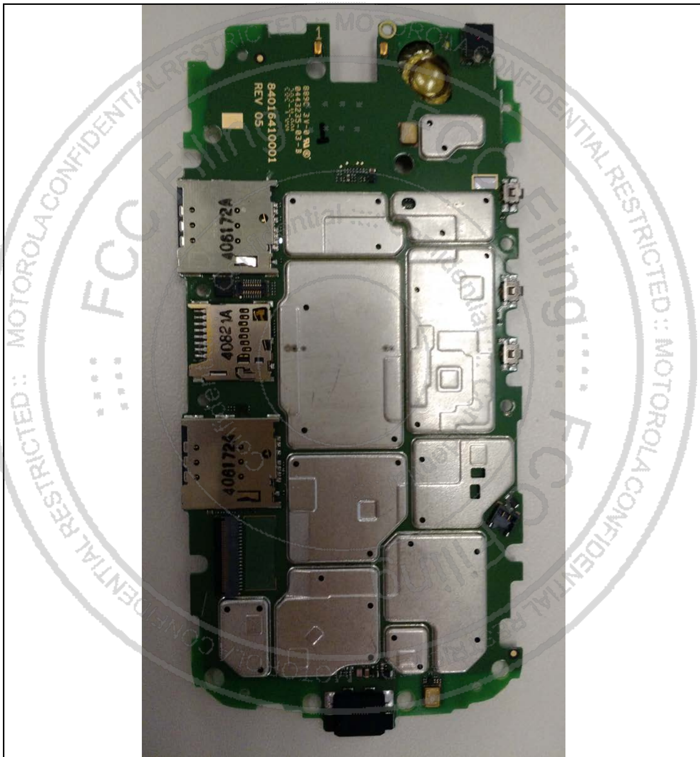
Photograph 9-1: Front side view of the device's PC Board, Shields in place.
