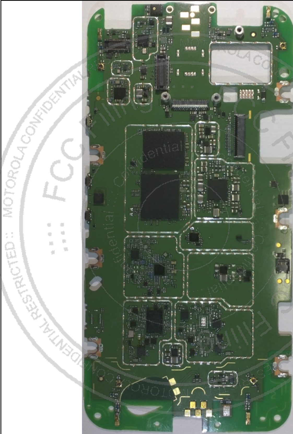
Photograph 9-3: Front side view of the device's PC Board, Shields Removed.
