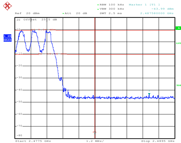
1Mbps Hopping Mode High Band Edge Plot
