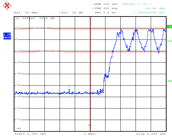
1Mbps Hopping Mode Low Band Edge Plot
