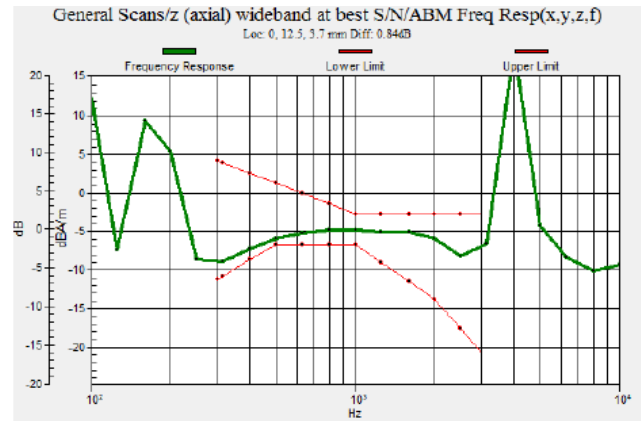
Fig 7.2 GSM1900 Ch661
