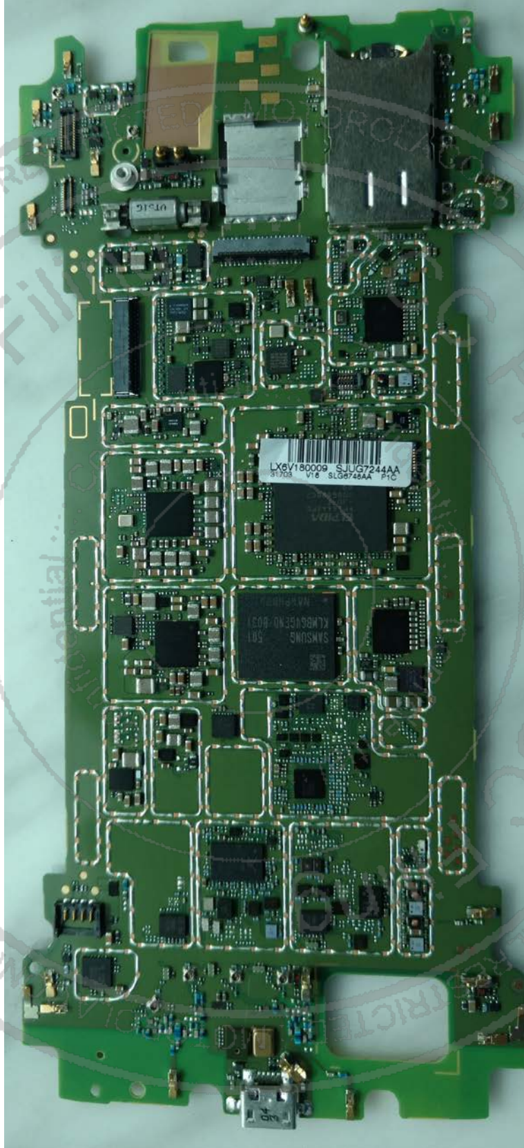
Photograph 9-3: Front side view of the device's PC Board, Shields Removed.
