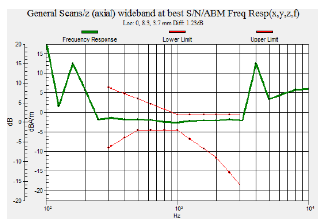
Fig 7.4 WCDMA Band IV Ch1413
