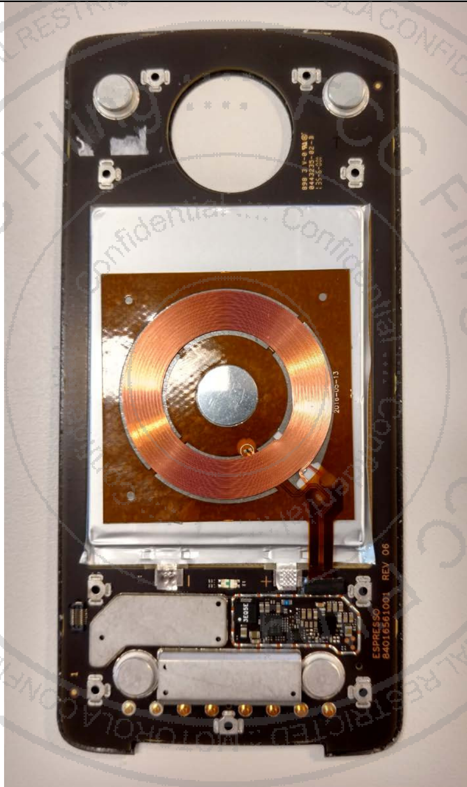
Photograph 9-1: Interior of Charging Accessory, featuring pick-up Coil.
