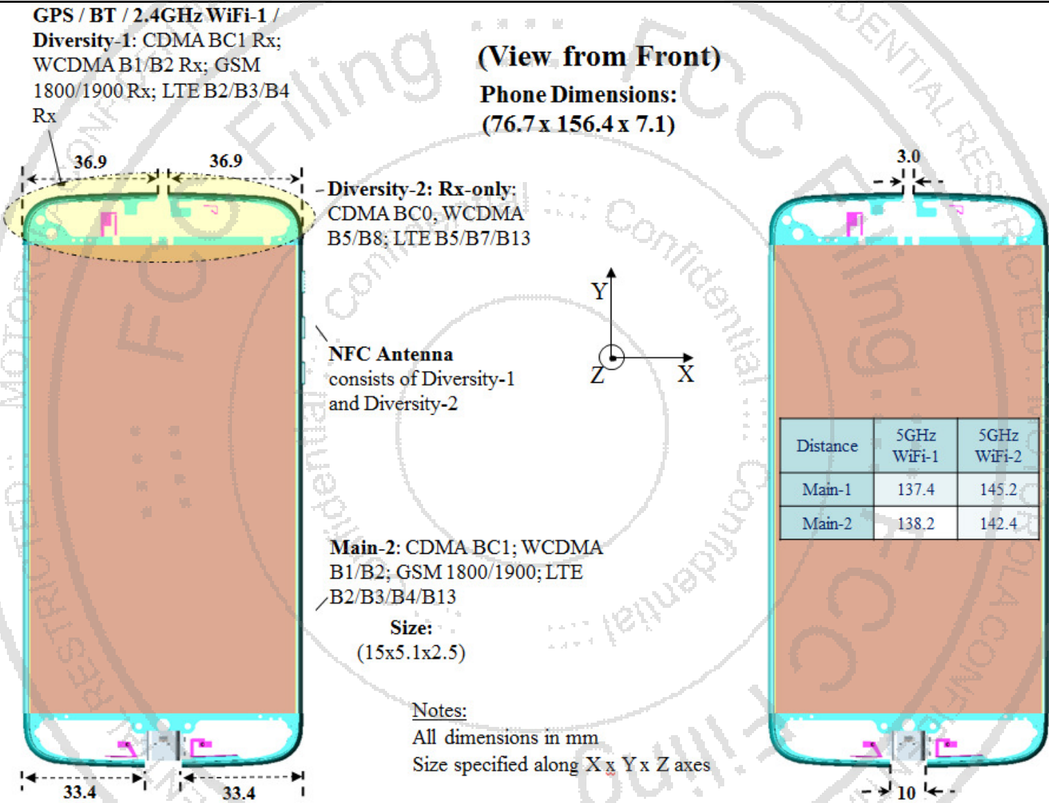
Photograph 9-6: Antenna Locations and Spacings.
