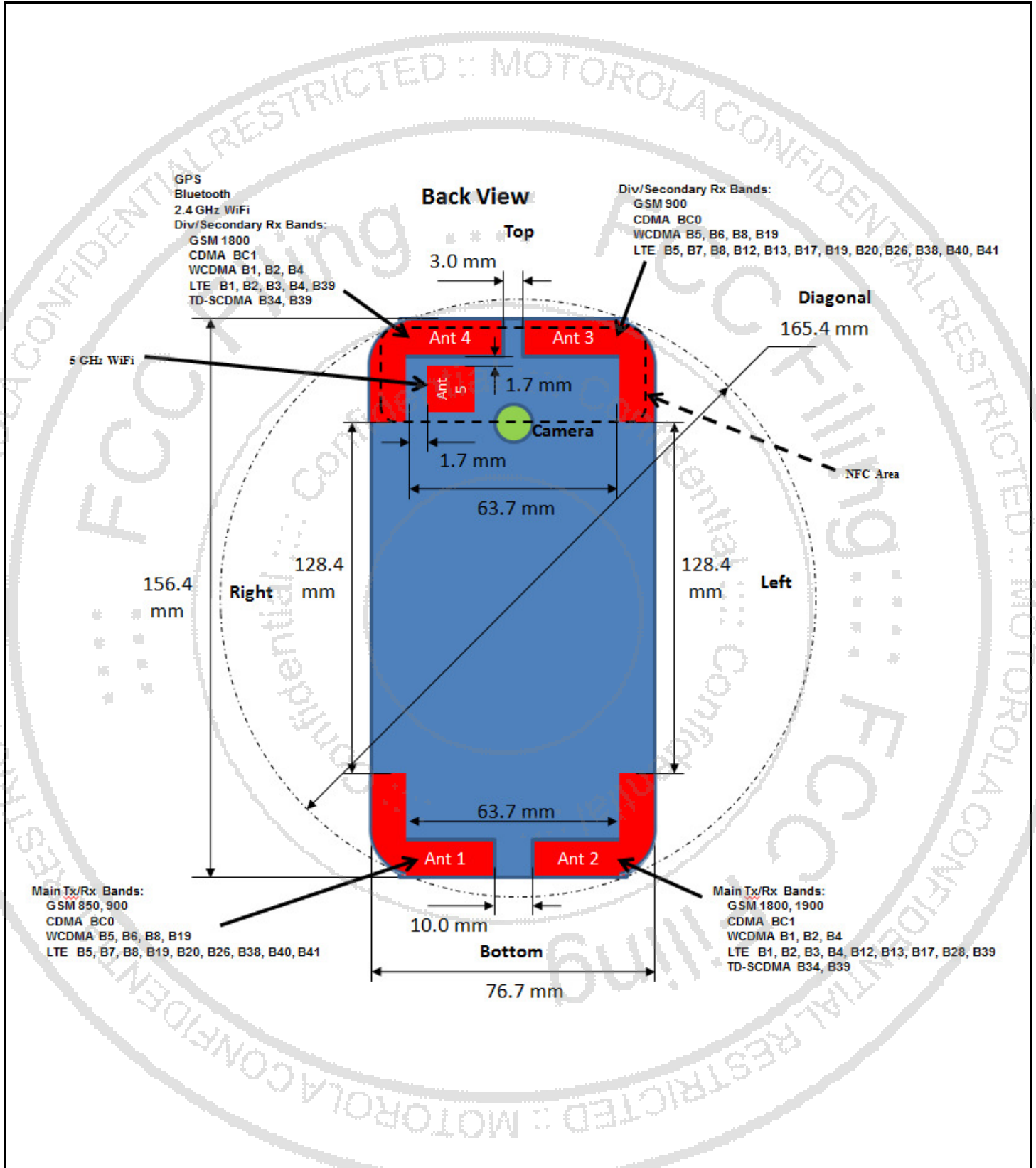
Photograph 9-5: Antenna Locations and Spacings.
